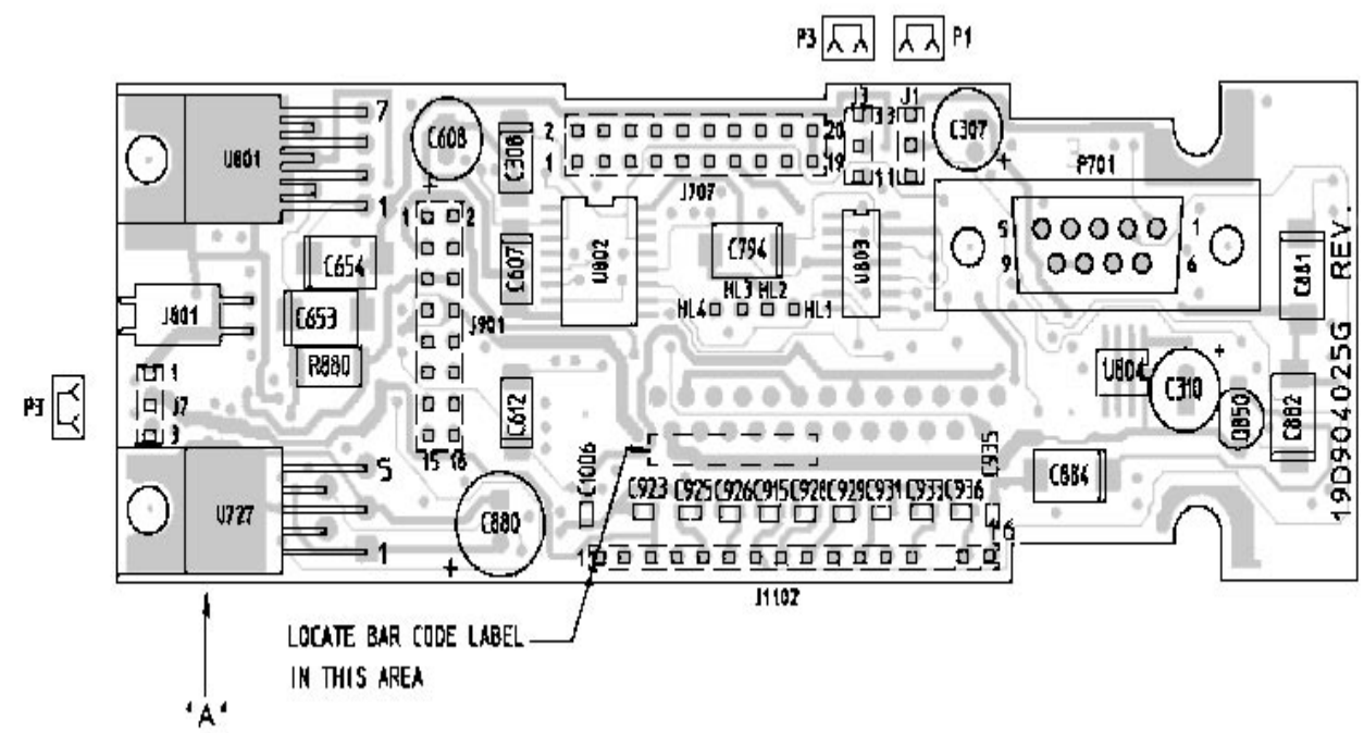
VIEW FROM COMPONENT SIDE
