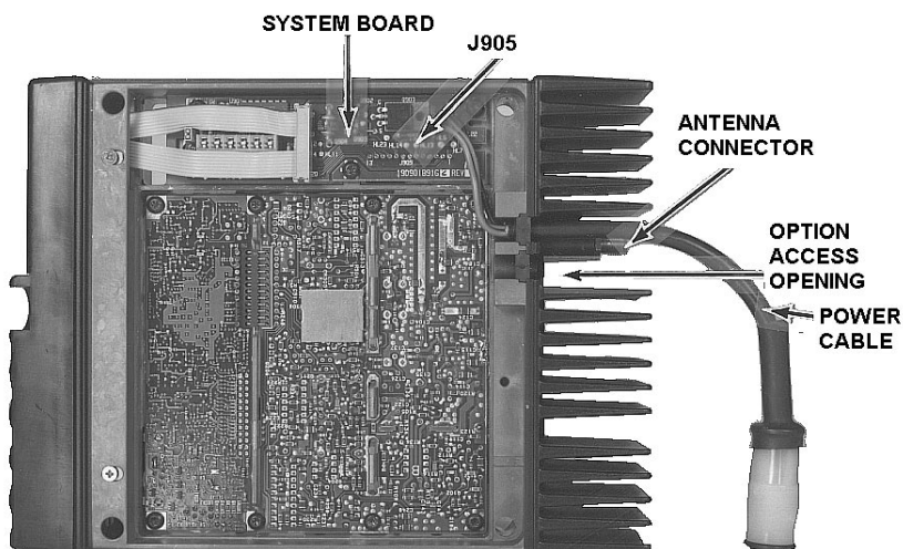
Figure 9 - Bottom View (Cover Removed)
