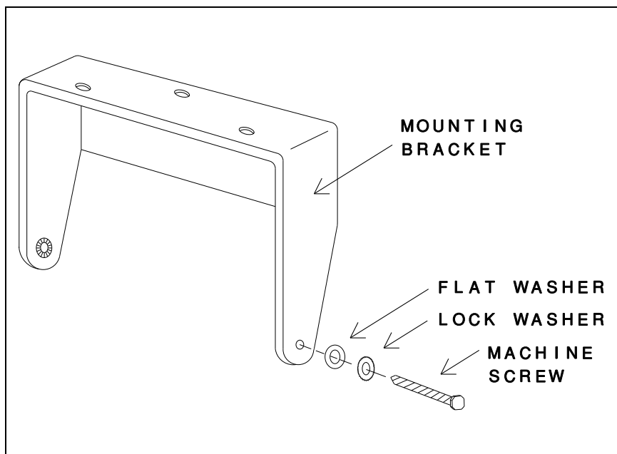
Figure 11 - Mounting The External Speaker
