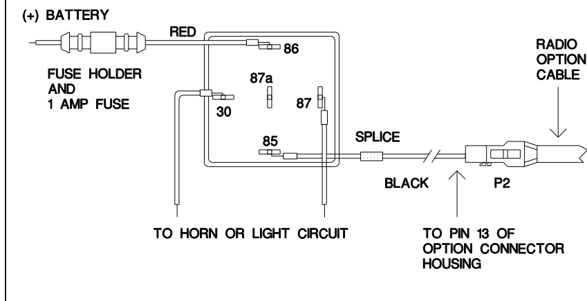
Figure 10 - External Alarm Relay
