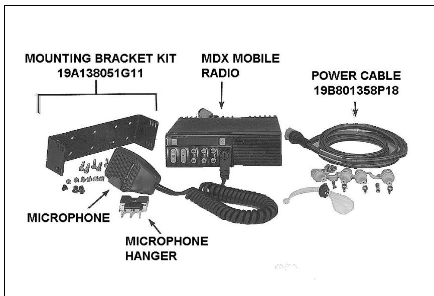
Figure 1 - MDX Components and Mounting Hardware
