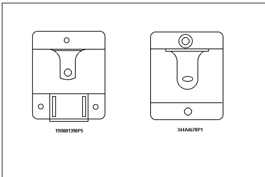
Figure 6 - Microphone Hanger
