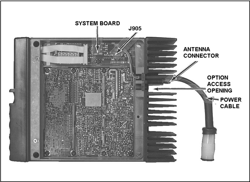
Figure 9 - Bottom View (Cover Removed)
