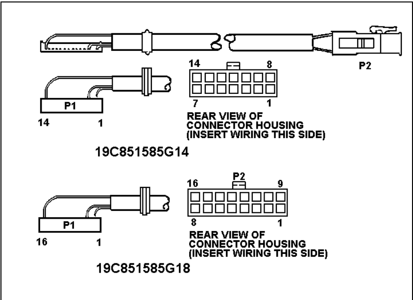
Figure 8- Option Cable Pin Locations
