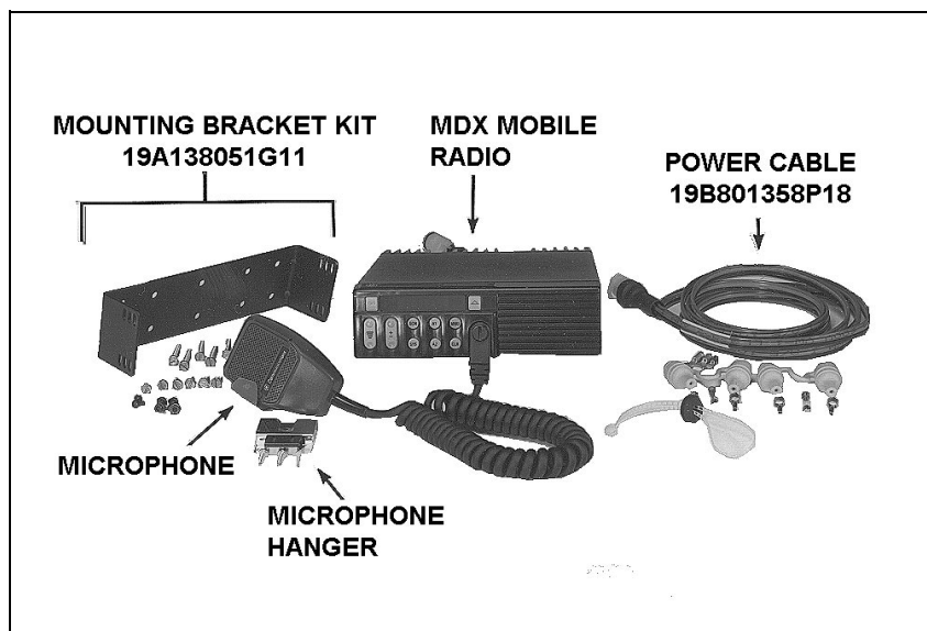
Figure 1 - MDX Components and Mounting Hardware
