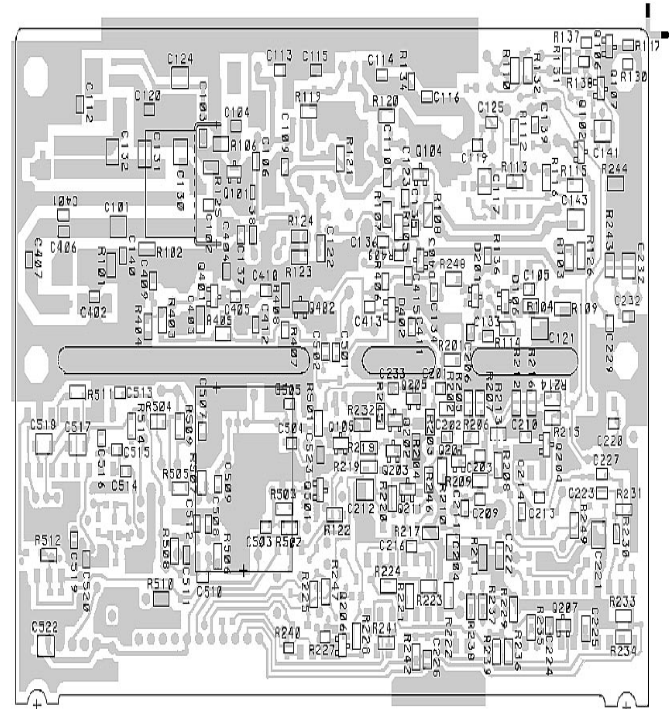
SOLDER SIDE
