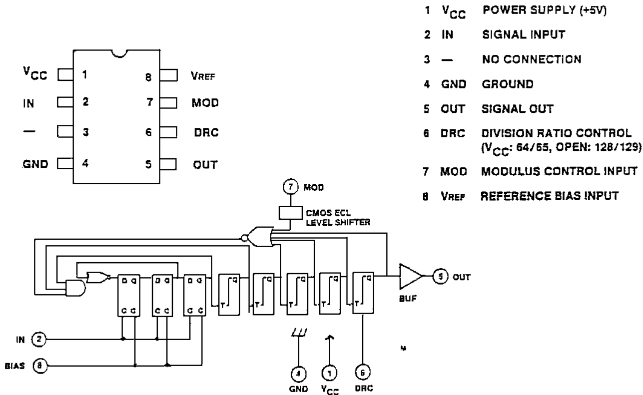
DIVIDER U205 19A704740P1
