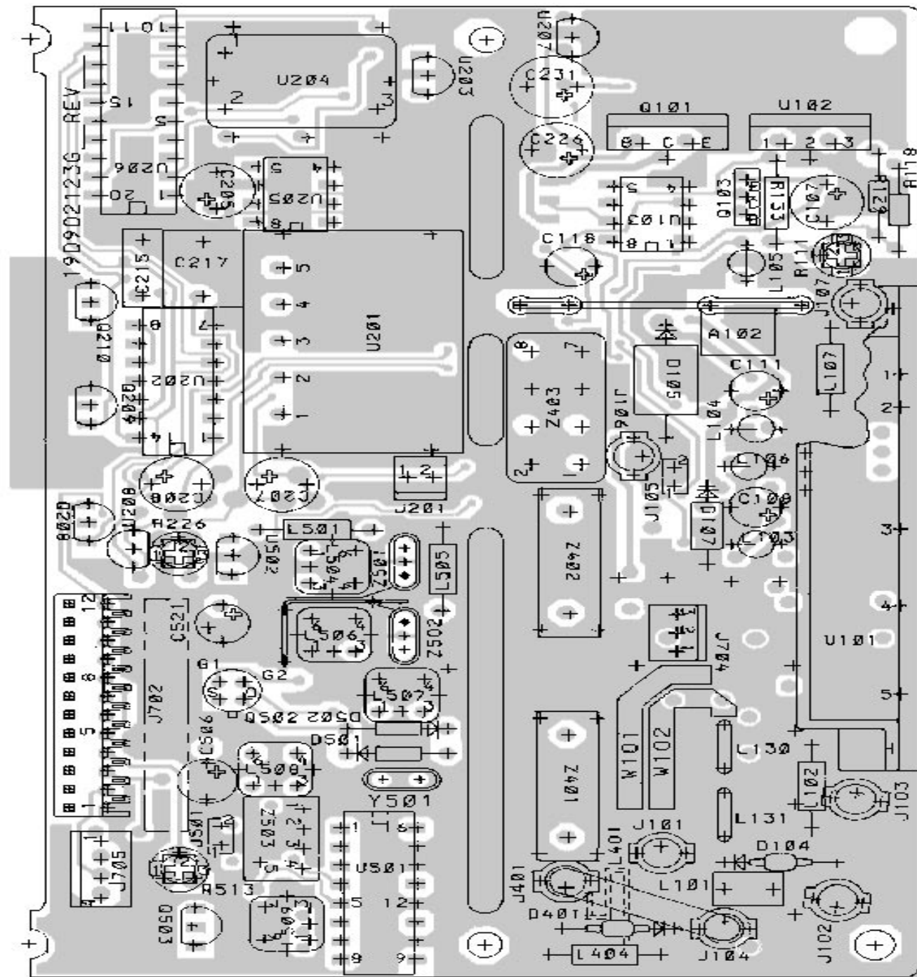
COMPONENT SIDE
