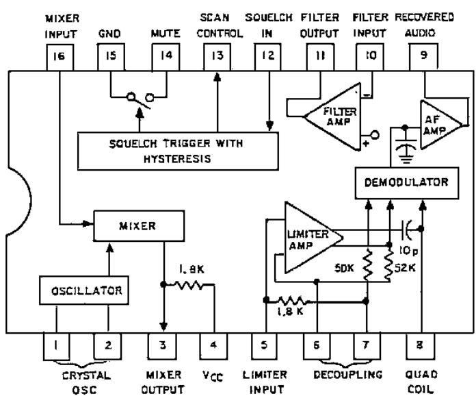
BLOCK DIAGRAM
