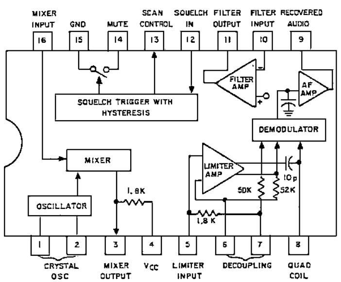
BLOCK DIAGRAM
