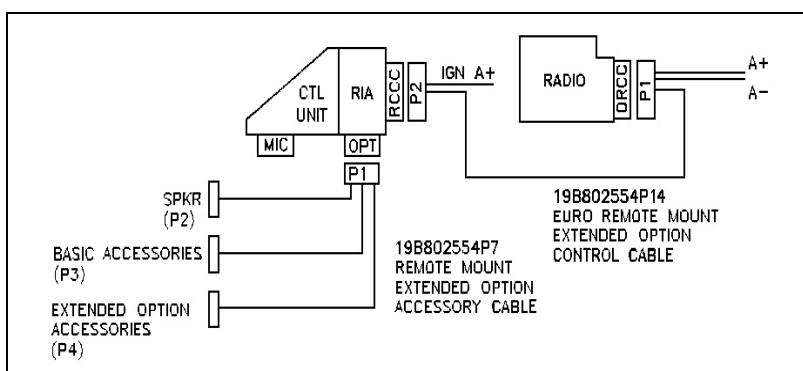
Figure 12 - Remote Mount Extended Option Accessory Interconnections (EURO Models Only)
