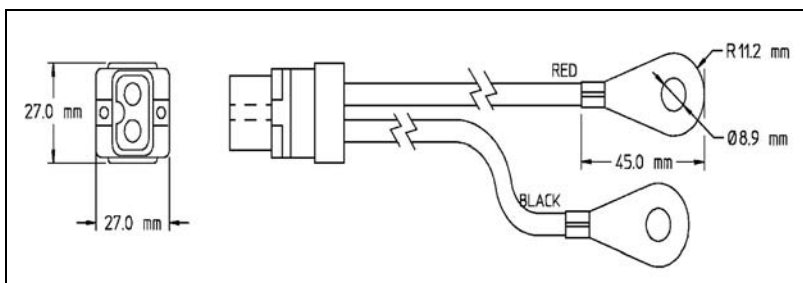
Figure 13 - Power Cable 19B802622P1 (USA Only)
