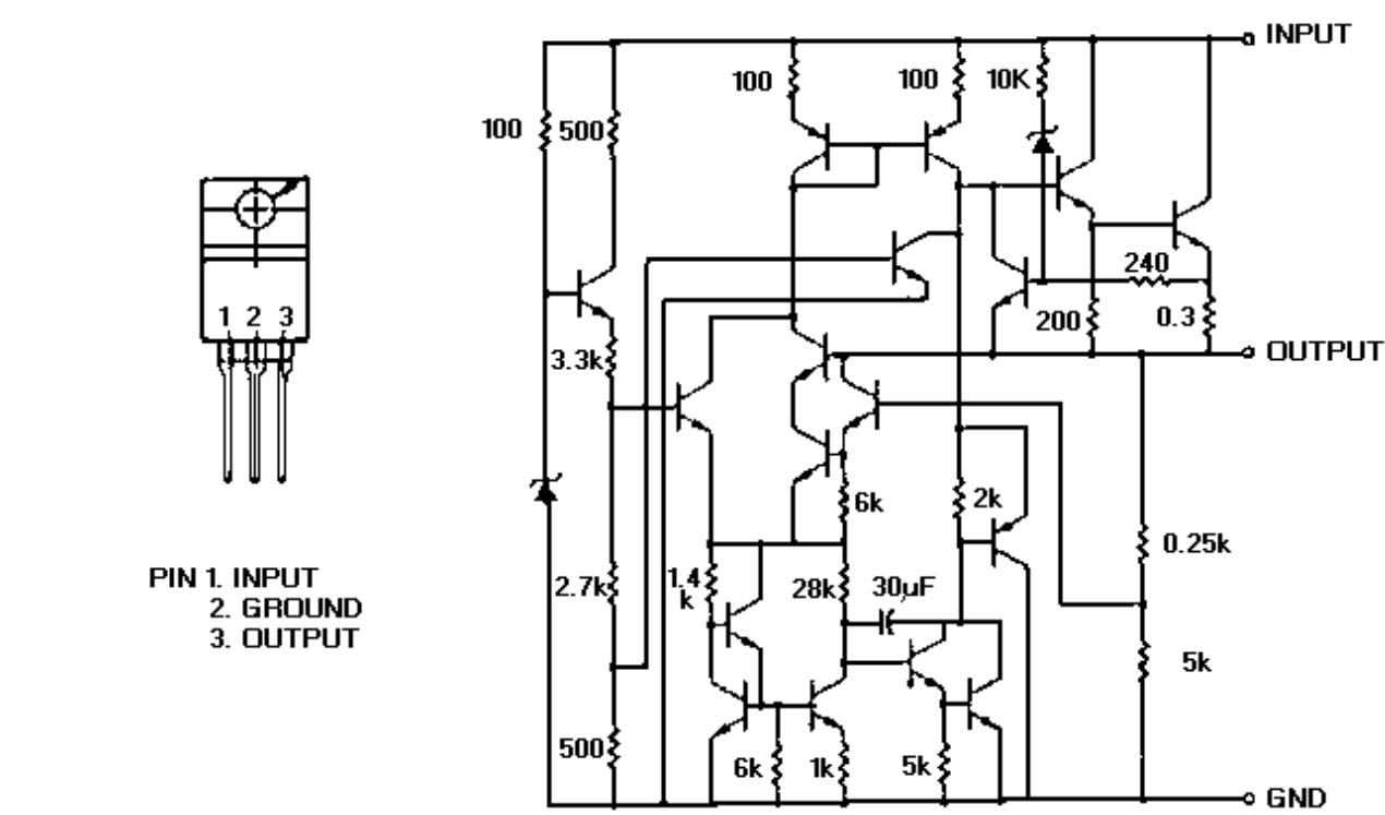
Reset Circuit IC610
