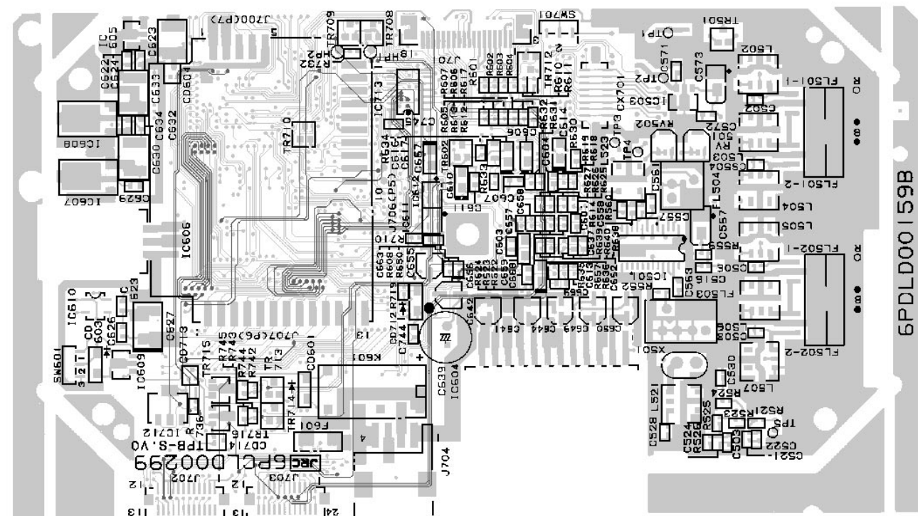
SOLDER SIDE
