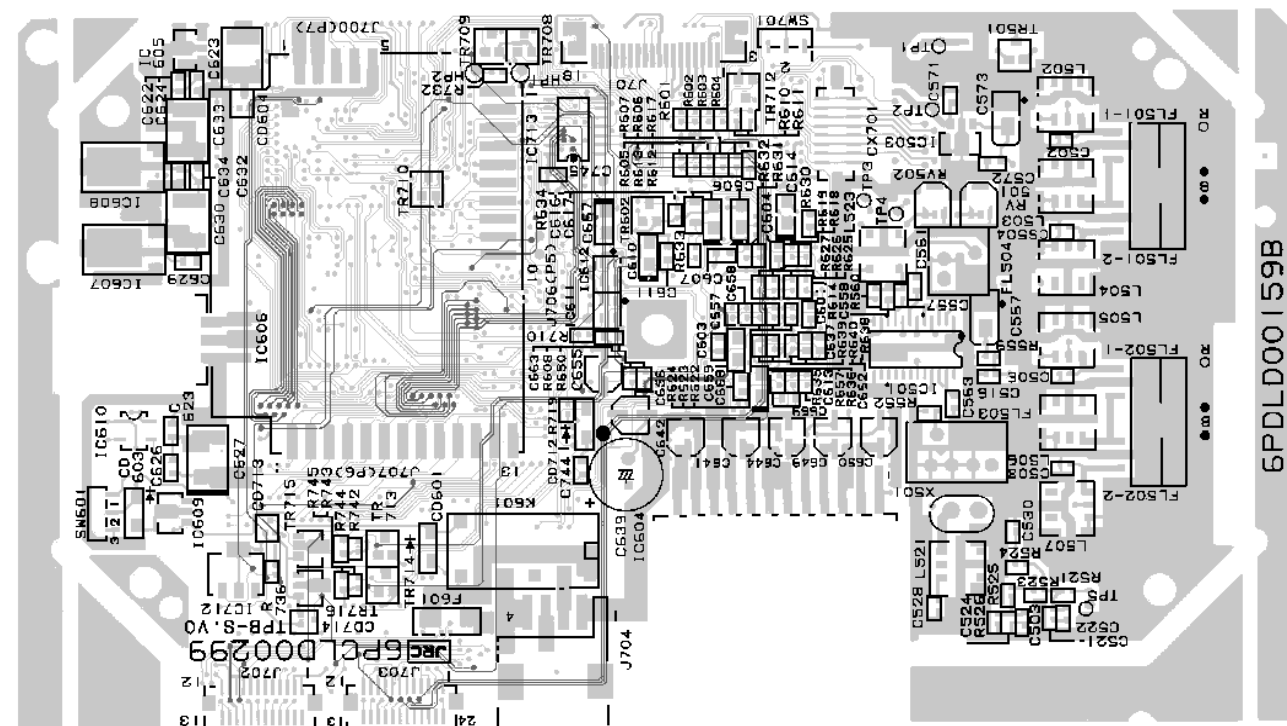
SOLDER SIDE
