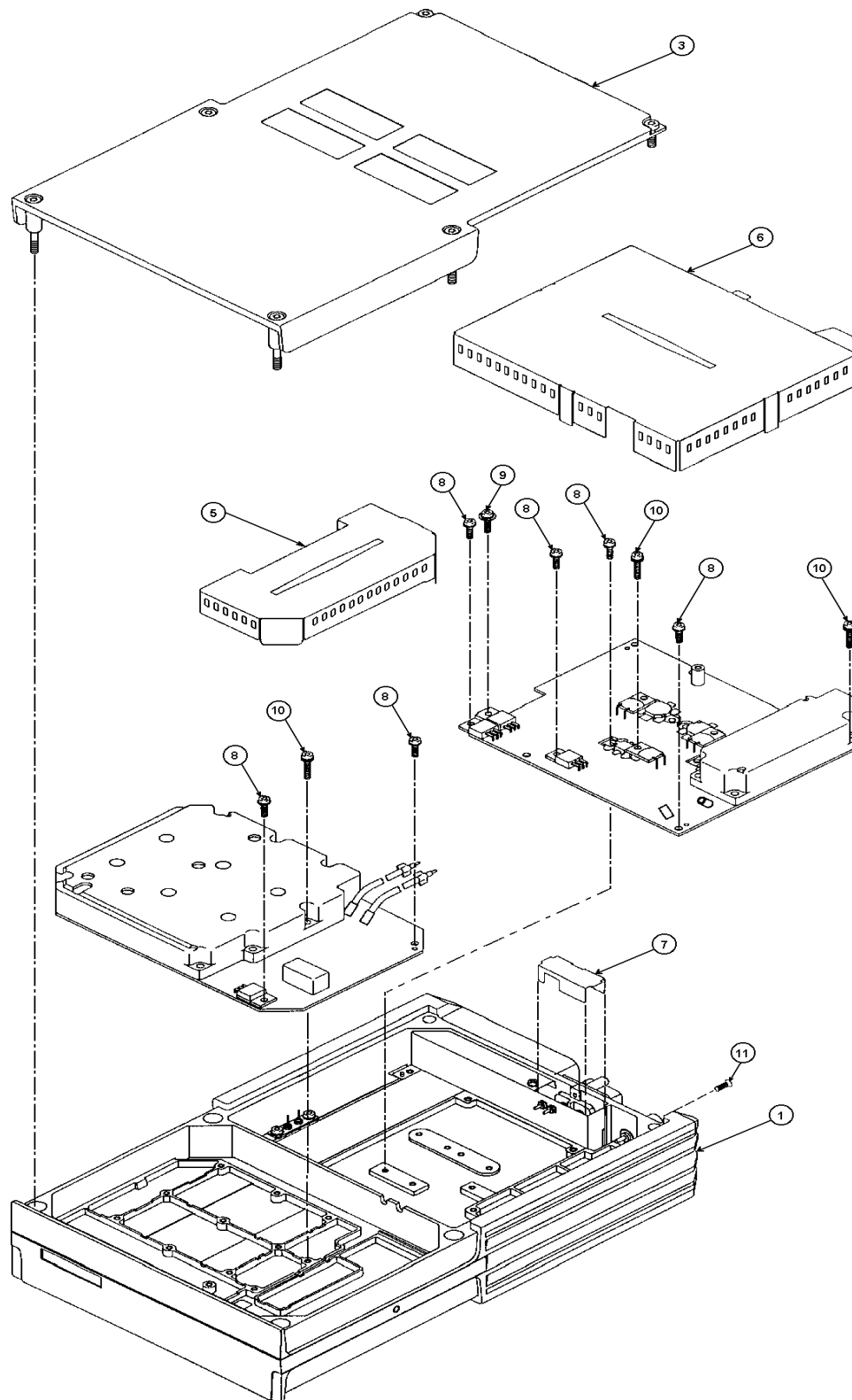
LOW BAND (EXPLODED VIEW AND PARTS LIST (1/2))
