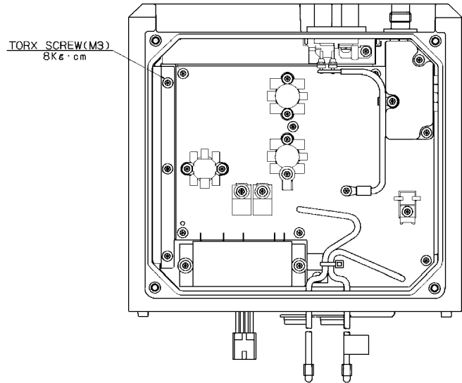
BOTTOM VIEW (REMOVE COVER AND SHIELD COVER)
