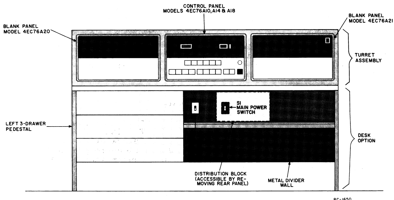
Figure 1 - Typical Radio Control Center
