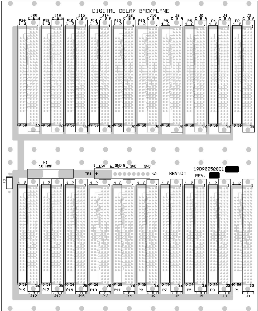
COMPONENT SIDE
