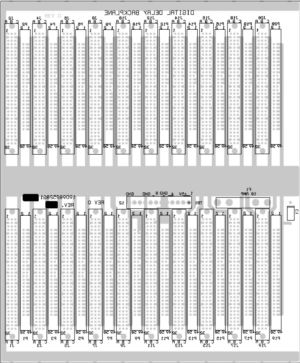
SOLDER SIDE
