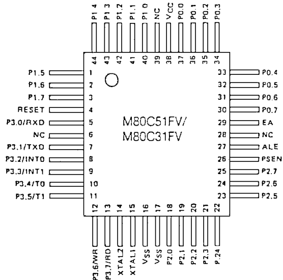
PIN IDENTIFICATION
