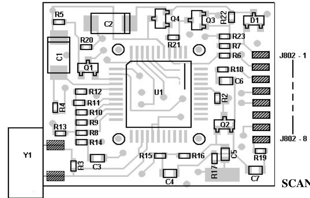
COMPONENT SIDE
