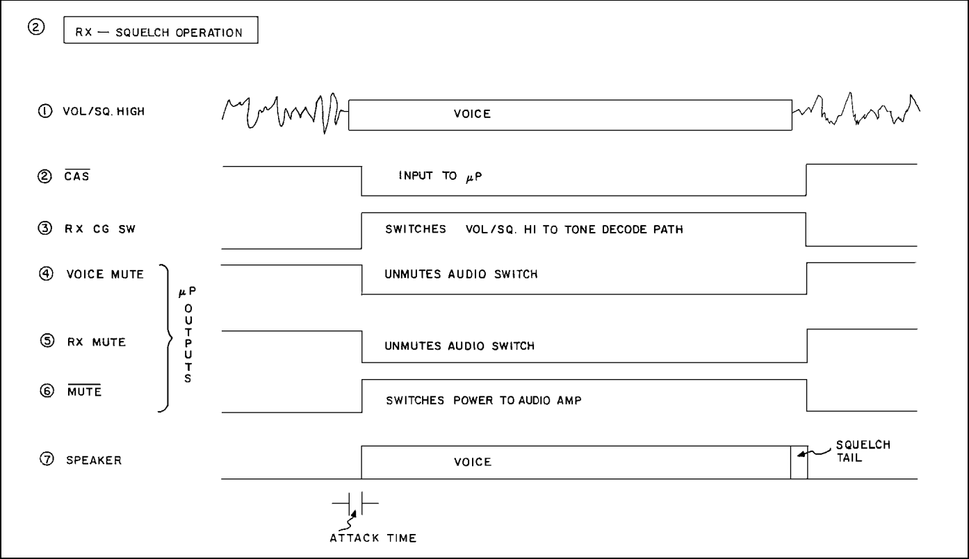
Figure 8 - RX Squelch Operation
