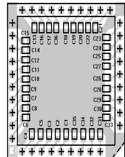
SPUR FILTER BOARD
