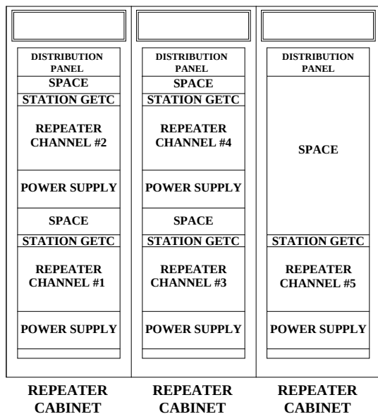
Figure 2 - Typical Five Channel Repeater Cabinet
