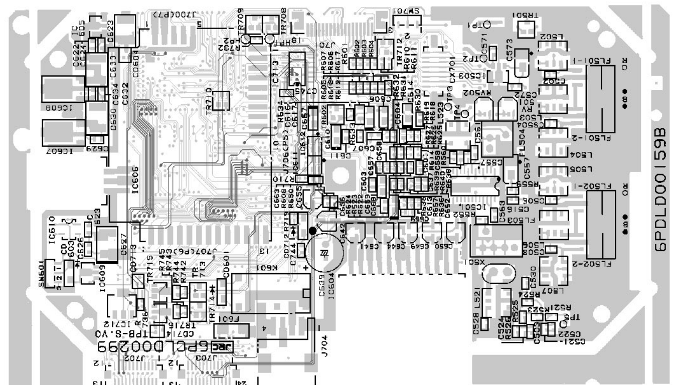
SOLDER SIDE
