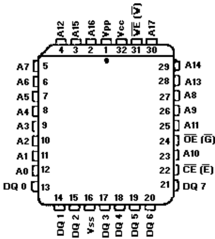
Flash Memory IC707
