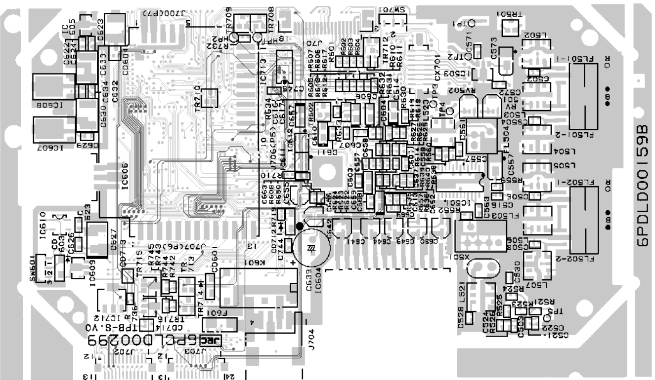
SOLDER SIDE
