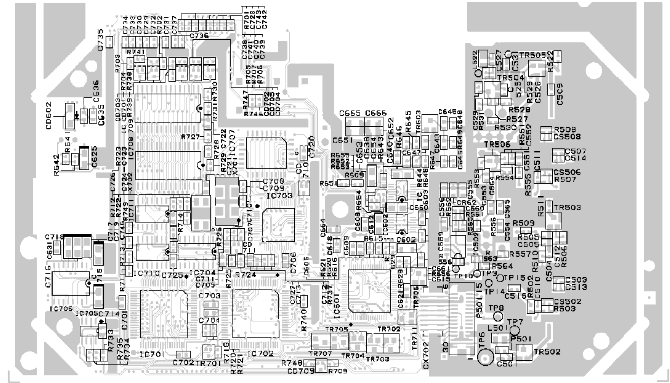
COMPONENT SIDE
