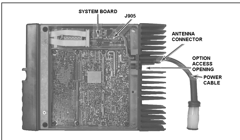
Figure 10 - Bottom View (Cover Removed)
