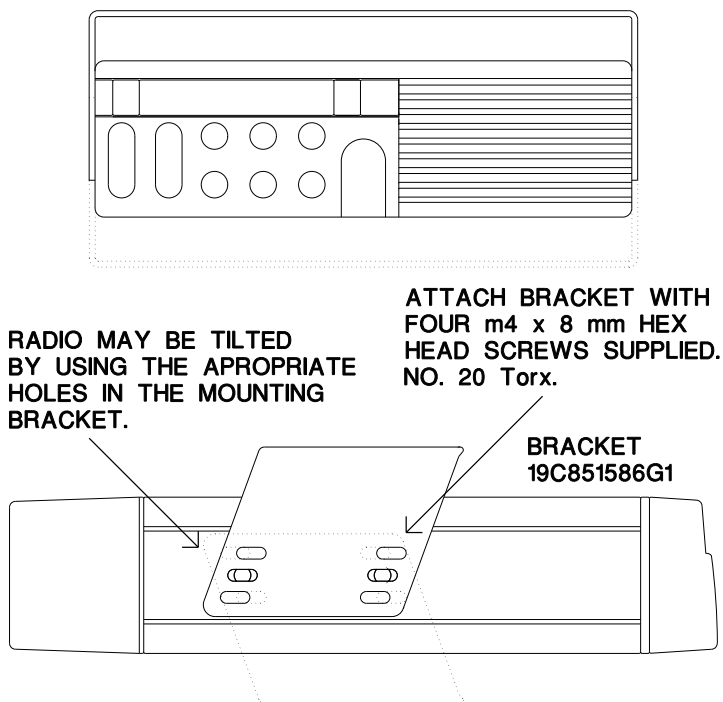
Figure 5 - Mounting Bracket Installation
