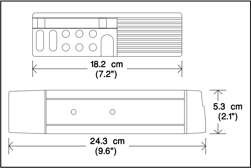
Figure 4 - Mounting Dimensions
