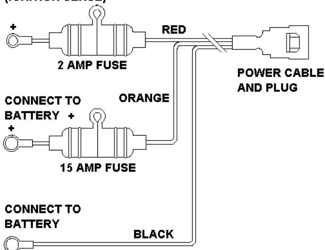
Figure 3 - Power Cable
