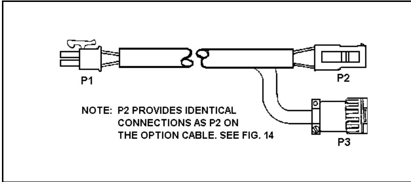
Figure 9 - Tone Cable Pin Location
