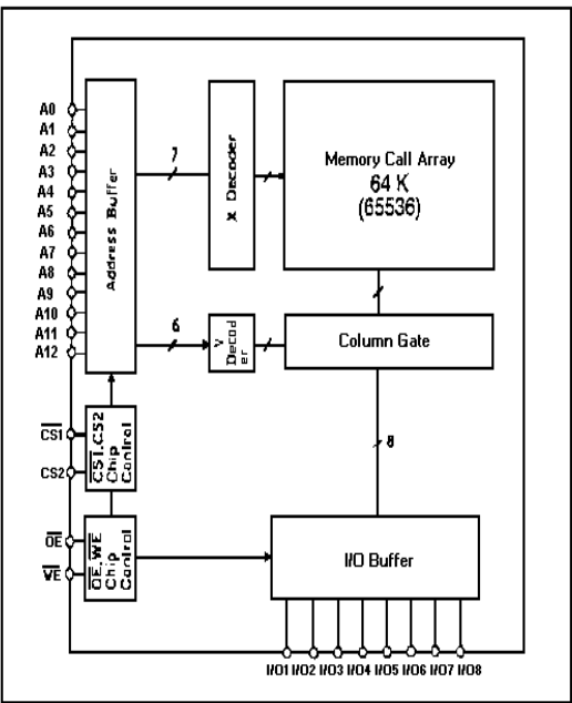
BLOCK DIAGRAM
