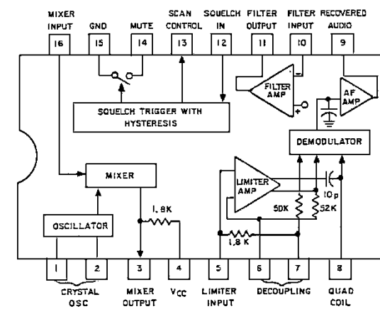
BLOCK DIAGRAM
