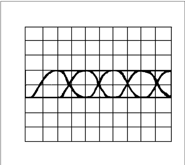
Figure 2 - High Speed Data Eye Pattern TEST EQUIPMENT AND SERVICE AIDS The following list of test equipment and service aids are available to facilitate servicing.
