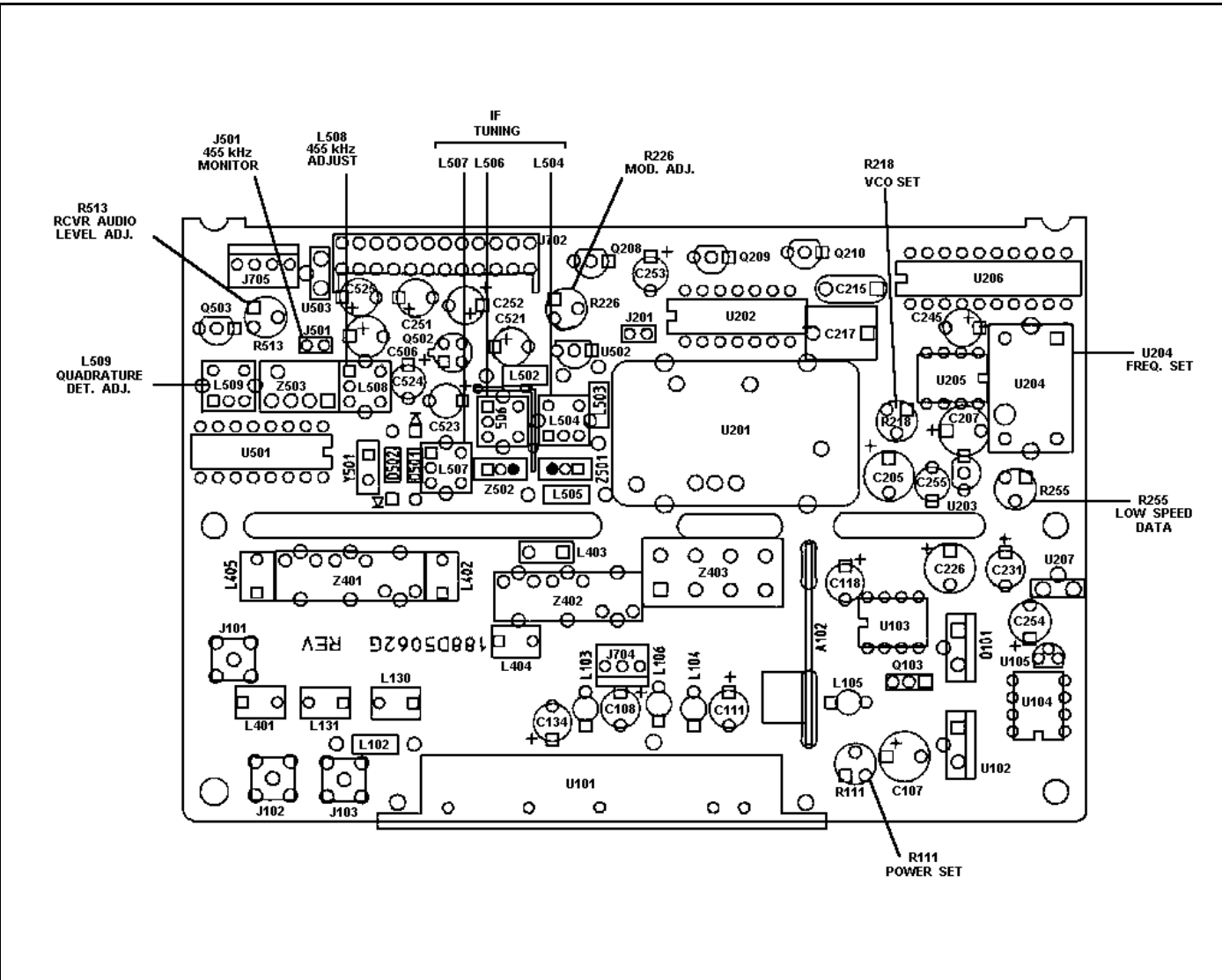
Figure 3 - Location Of Controls And Adjustments, RF Board
