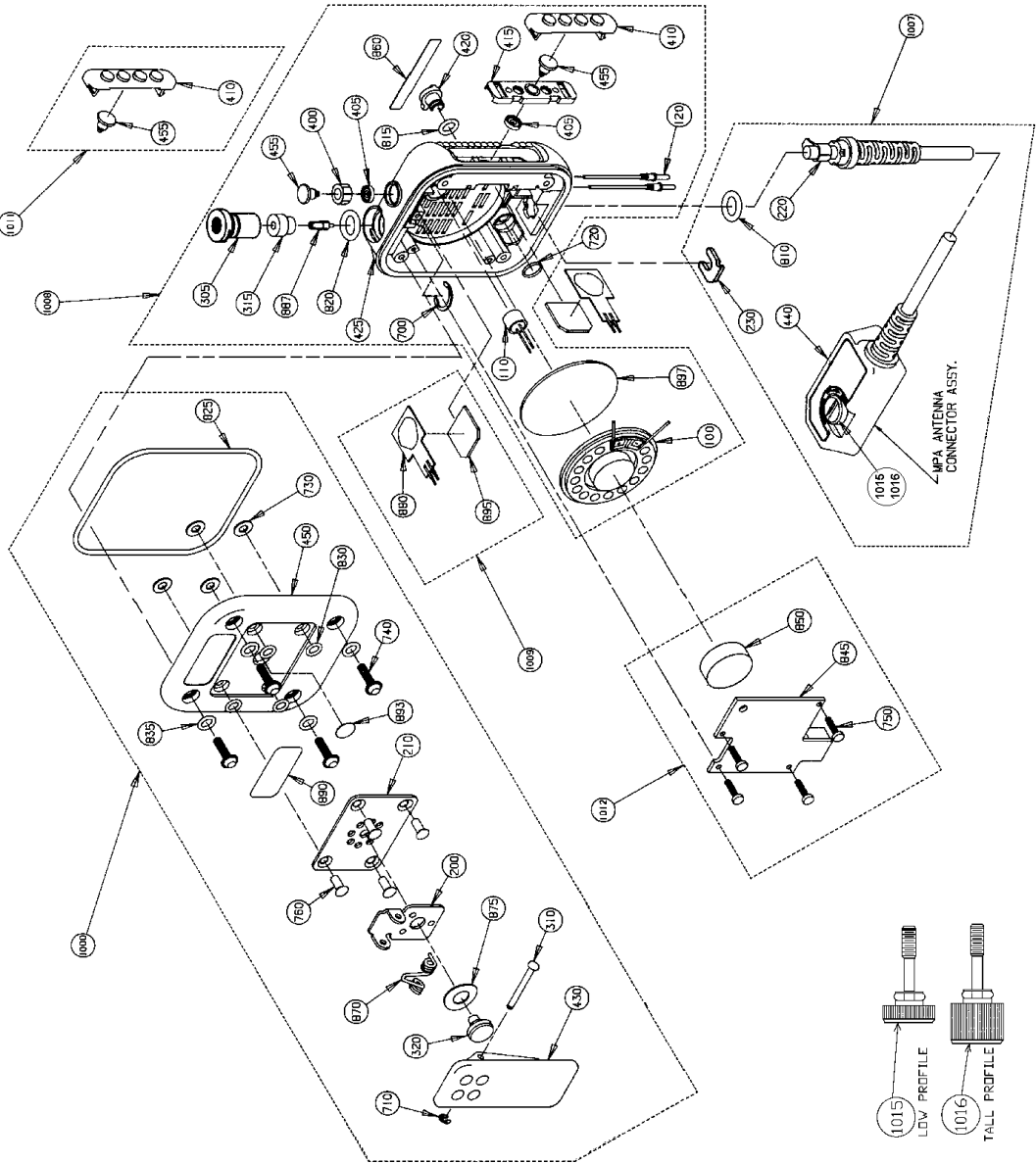
M-PA SPEAKER/MIC/ANTENNA 344A4189P12 & P14
