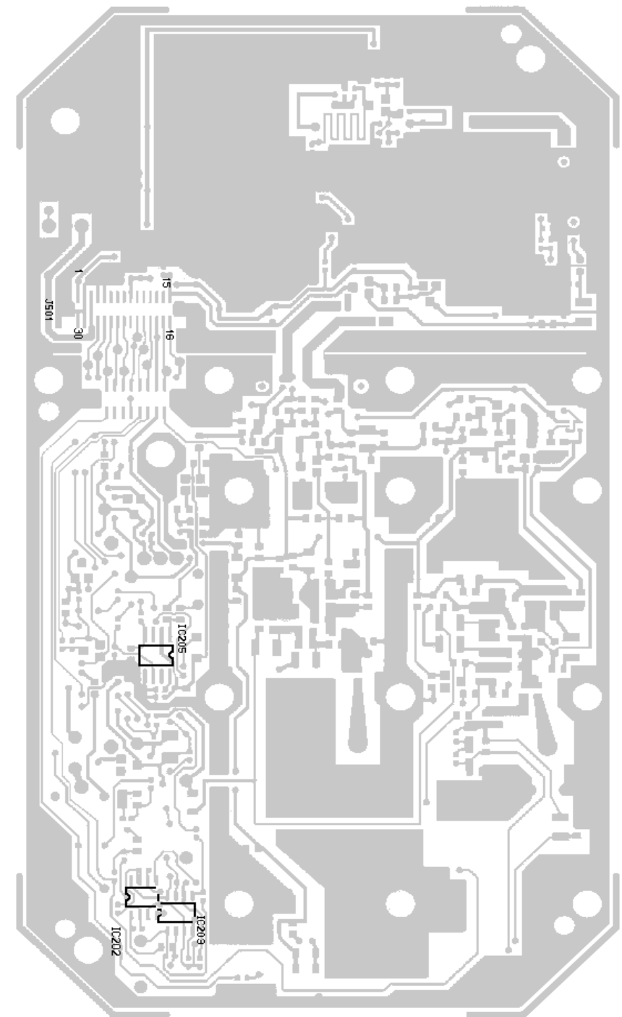
ORION 800 MHz SYNTHESIZER/RECEIVER/EXCITER
