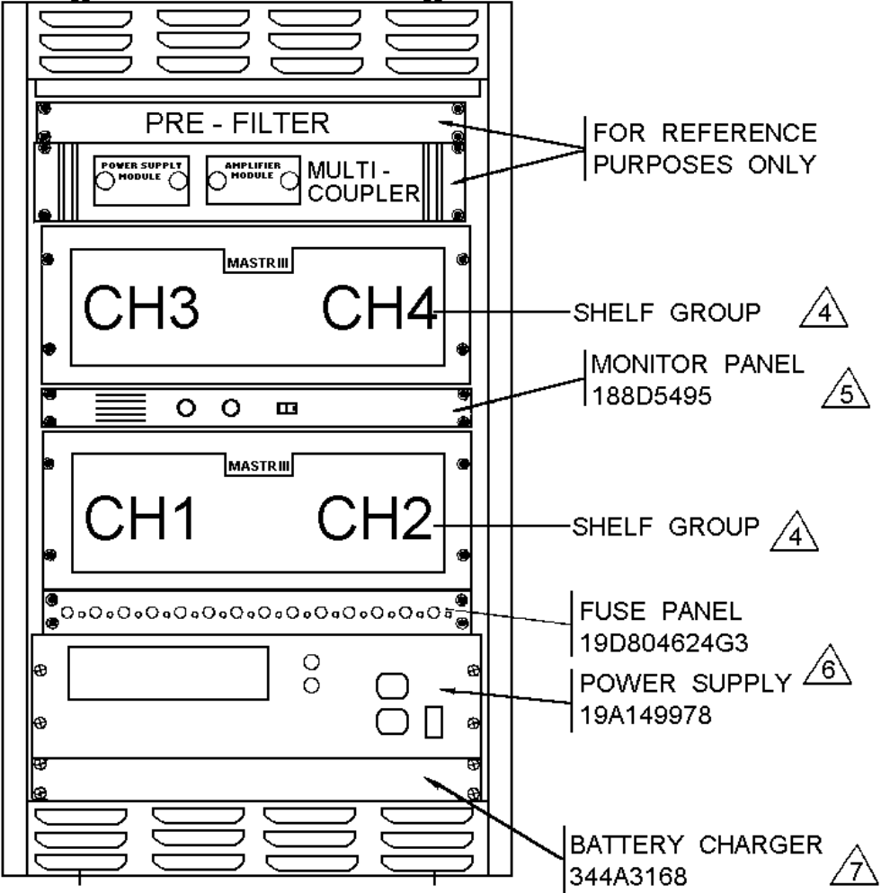
FRONT VIEW
