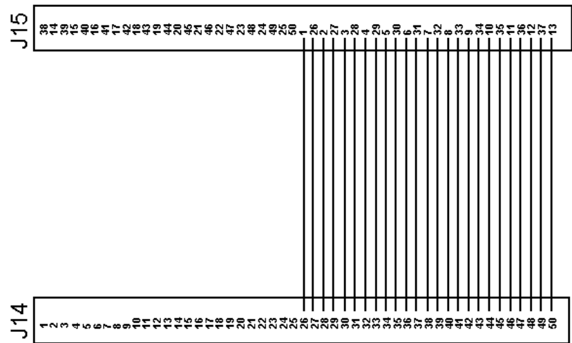
WIRING DIAGRAM
