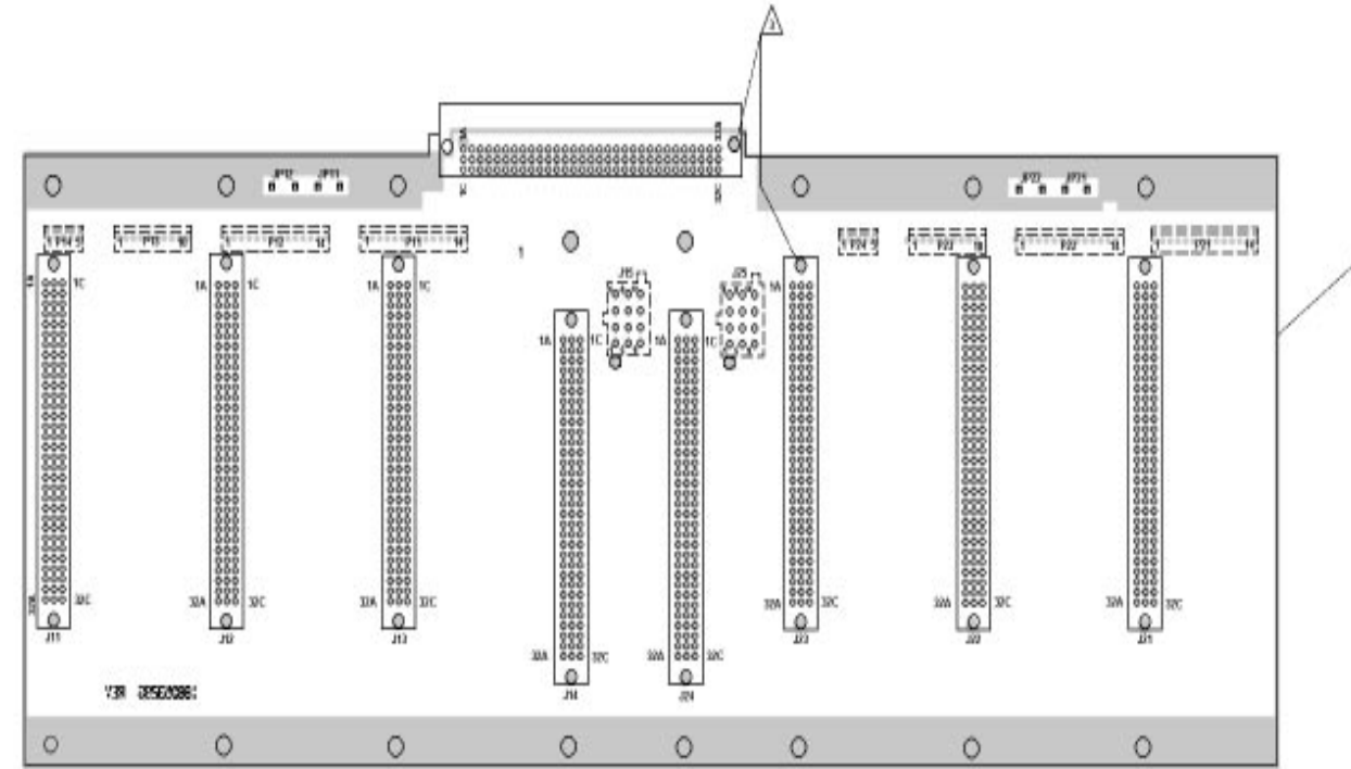
Backplane Board 188D5329G1
