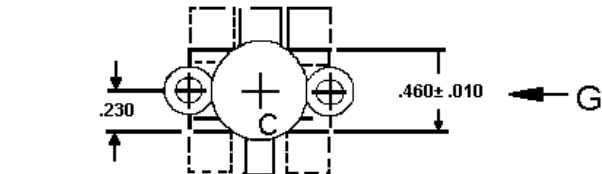
DETAIL F LEAD TRIMMING FOR Q1 THRU Q3 G3 USE EGE TOOL #423445 G1C FOR Q101 THRU Q103, G1 USE EGE TOOL #902/97 -G1A (TAKEN FROM SHEET 1)
