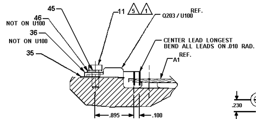
SECTION C - C (TAKEN FROM SHEET 1) LEAD FORMING AND HARDWARE STACKUP FOR Q203 & U100 FOR Q203, U100 USE TOOL #423445G1A
