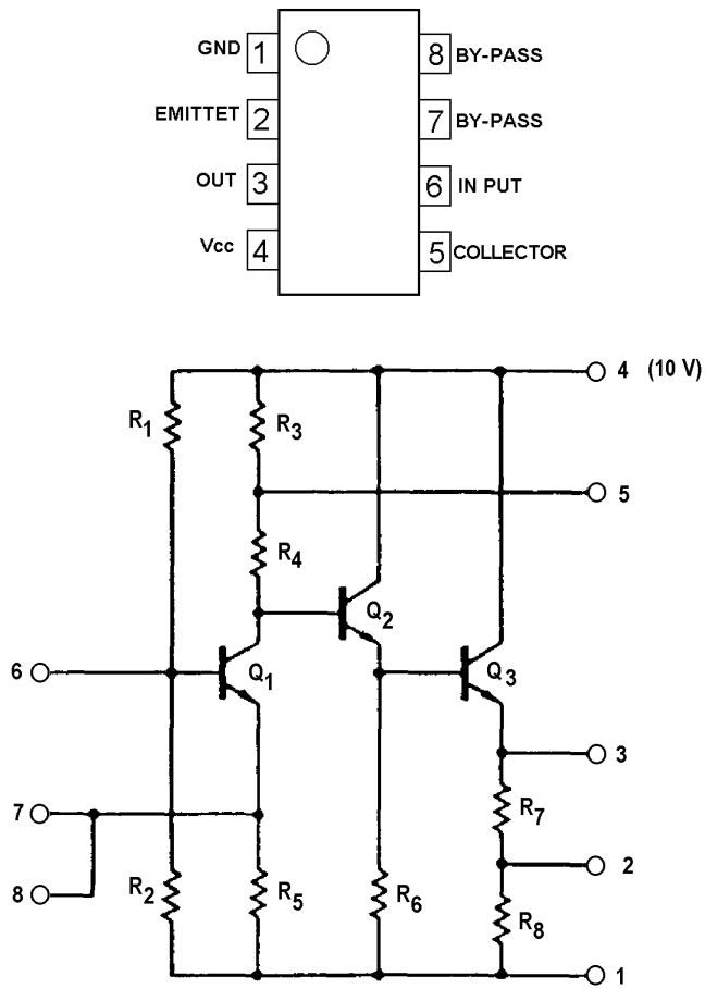
Linear, Wide Band Amplifier IC1 (NEC PC1658G)
