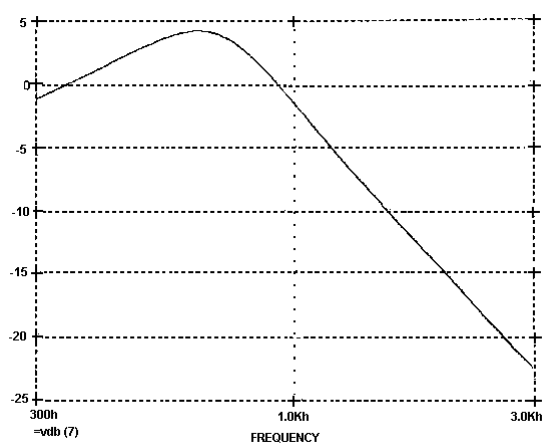
Figure 4 - Battery Alarm/Morse Code Band-Pass Filter
