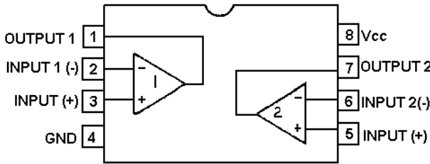
PIN CONNECTIONS
