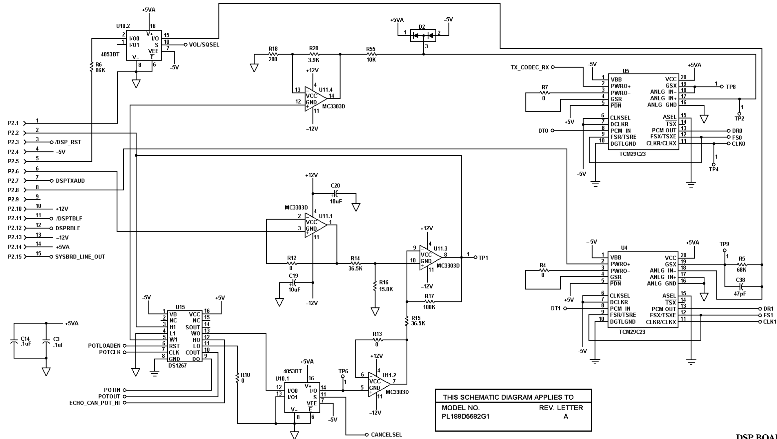
DSP BOARD 188D5682G1
