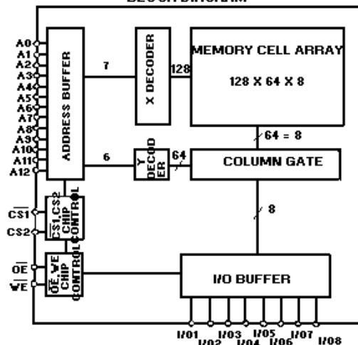
BLOCK DIAGRAM
