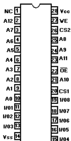
PIN ARRANGEMENT
