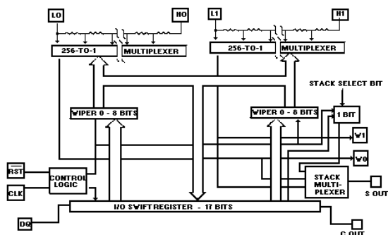
BLOCK DIAGRAM
