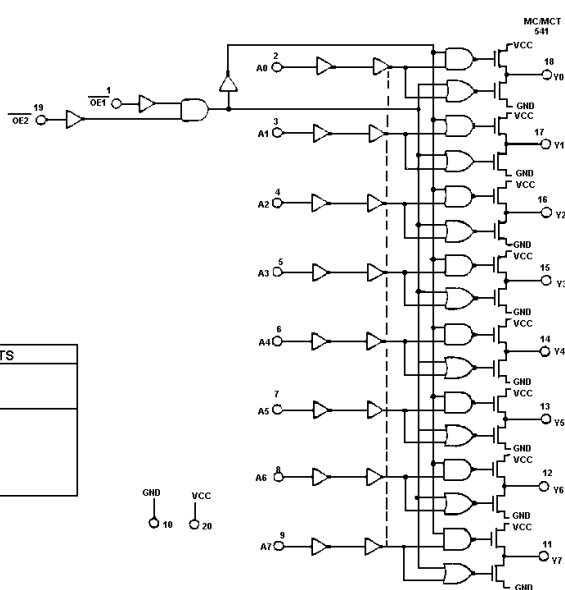
BLOCK DIAGRAM
