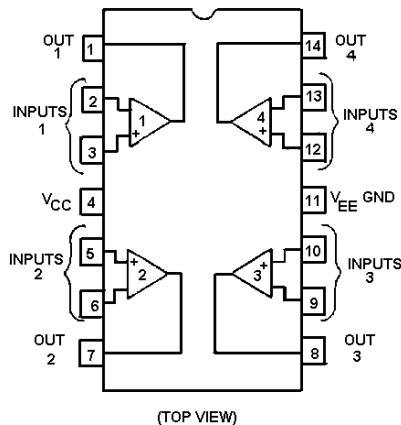
PIN CONNECTIONS
