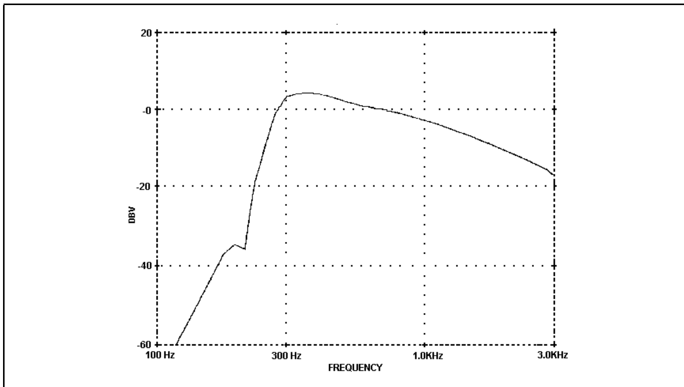
Figure 1 - Channel Guard Tone Reject (+1, -3 dBV)
