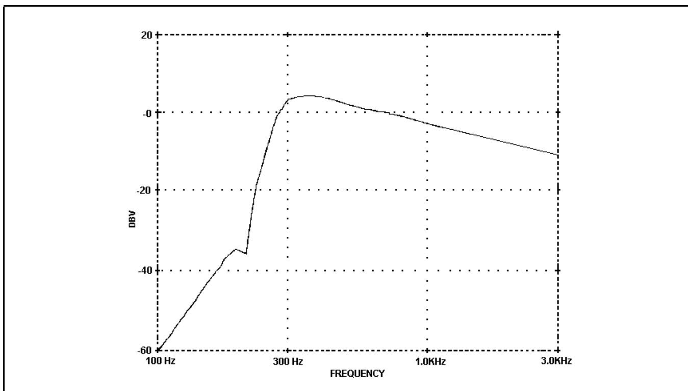
Figure 2 - Channel Guard Tone Reject Filter (+2, -8dBV)
