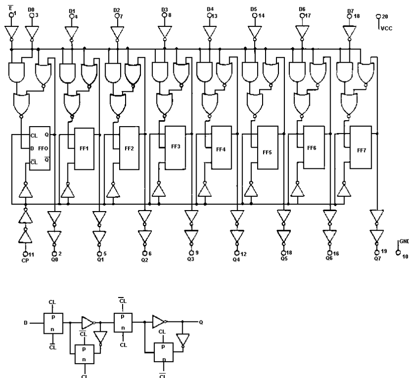
BLOCK DIAGRAM
