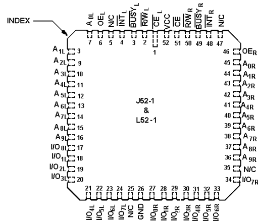
52-PIN LCC/PLCC TOP VIEW
