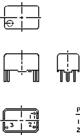
PIN CONNECTIONS 1. COMMON AND CASE 2. OUTPUT 3. + Vcc
