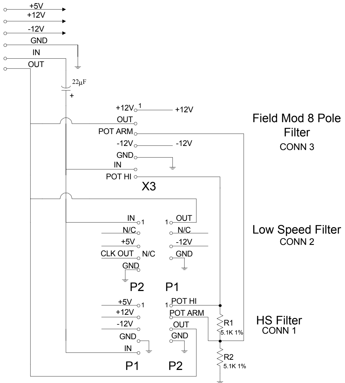
Filter Test Fixture
