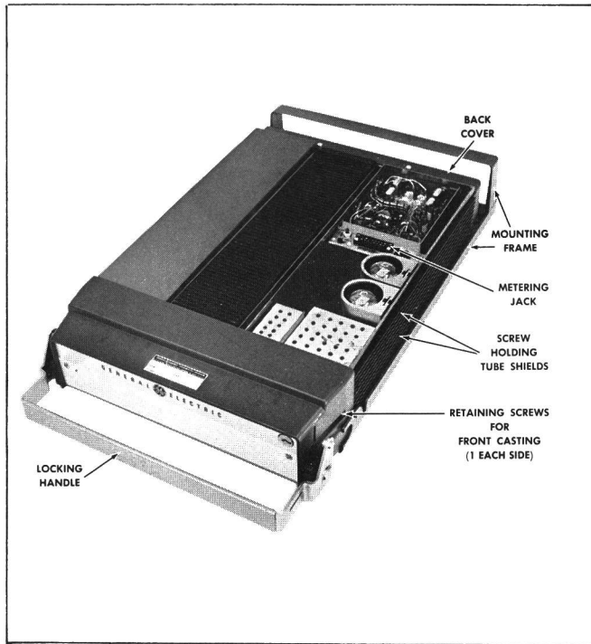
Figure 2 - Top Cover Removed
