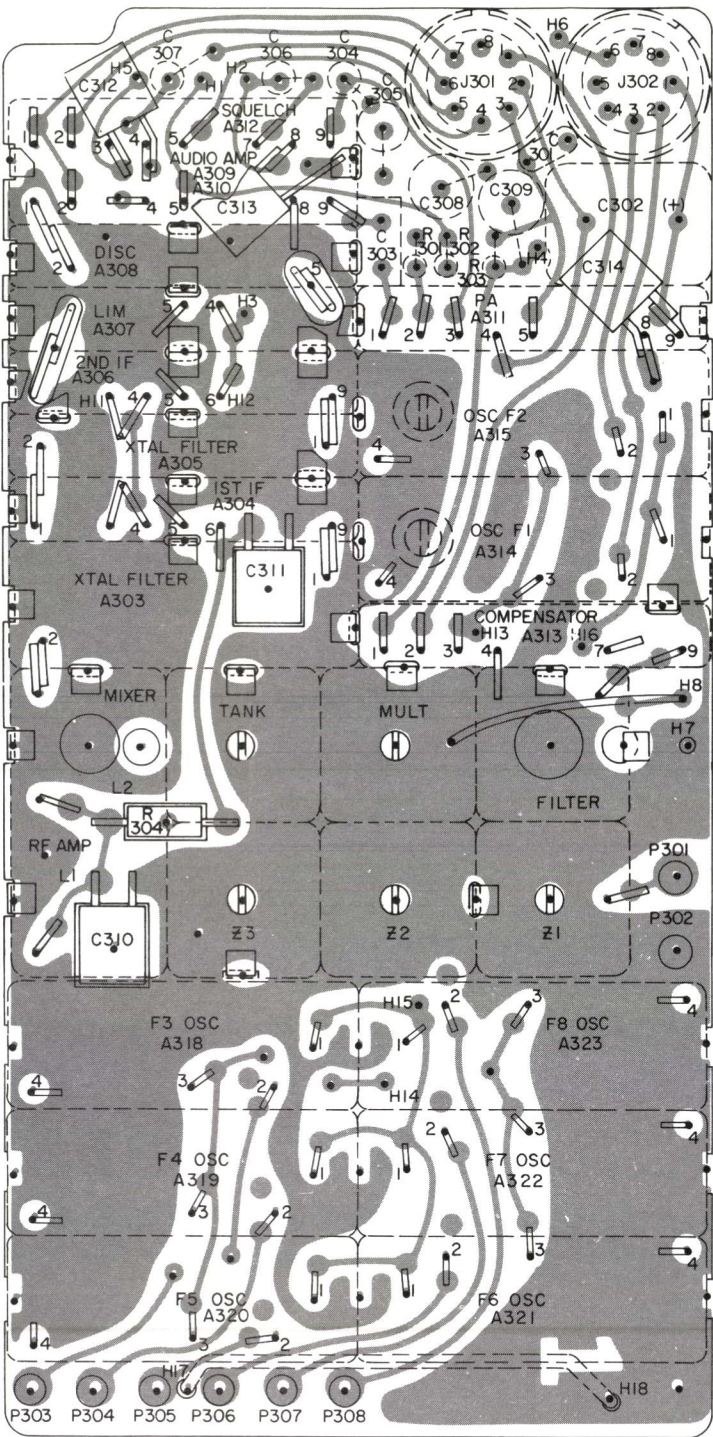
SOLDER SIDE
