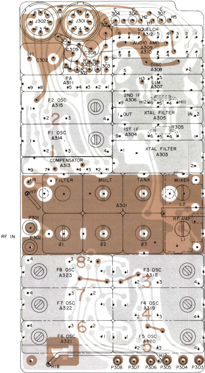
COMPONENT SIDE
