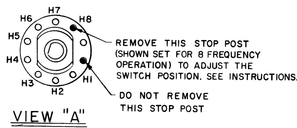
Figure 1 - Stop Post Adjustment
