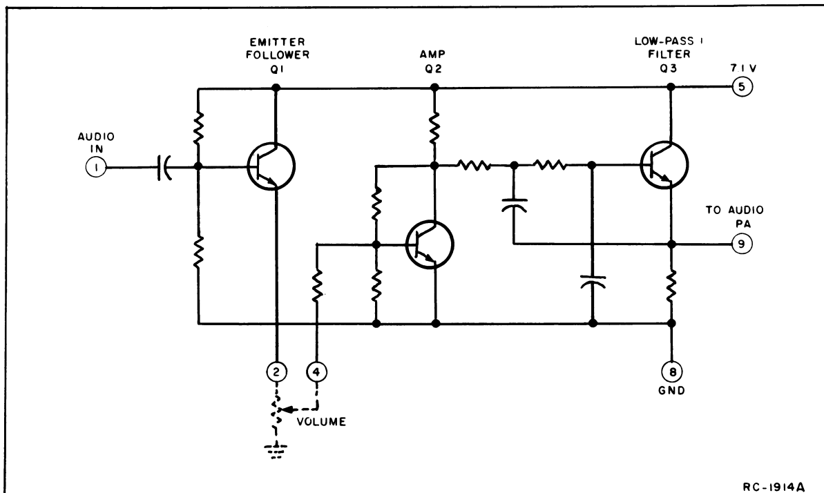
Figure 13 - Typical Audio Amplifier
