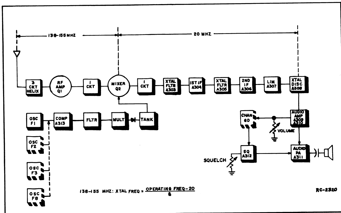
Figure 10 - Receiver Block Diagram
