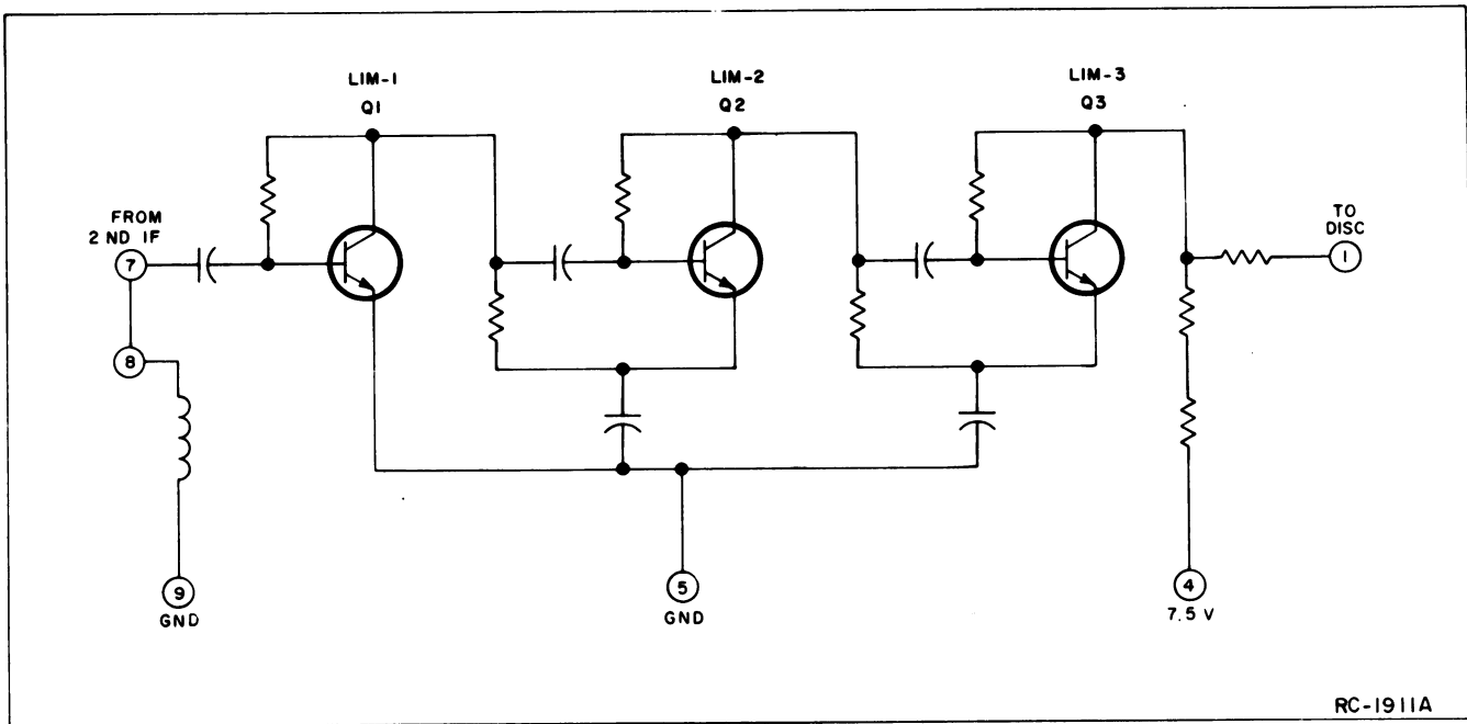
Figure 12 - Typical Limiter Circuit
