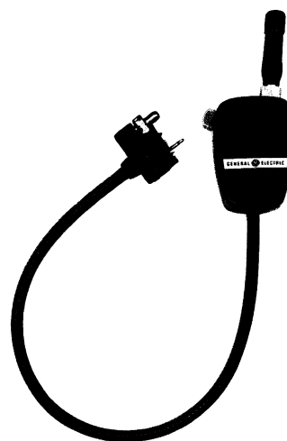
Remote Speaker-Microphone 4EM33H14 (Velcro® Hanger) 4EM33H15 (Hang-up Button)
