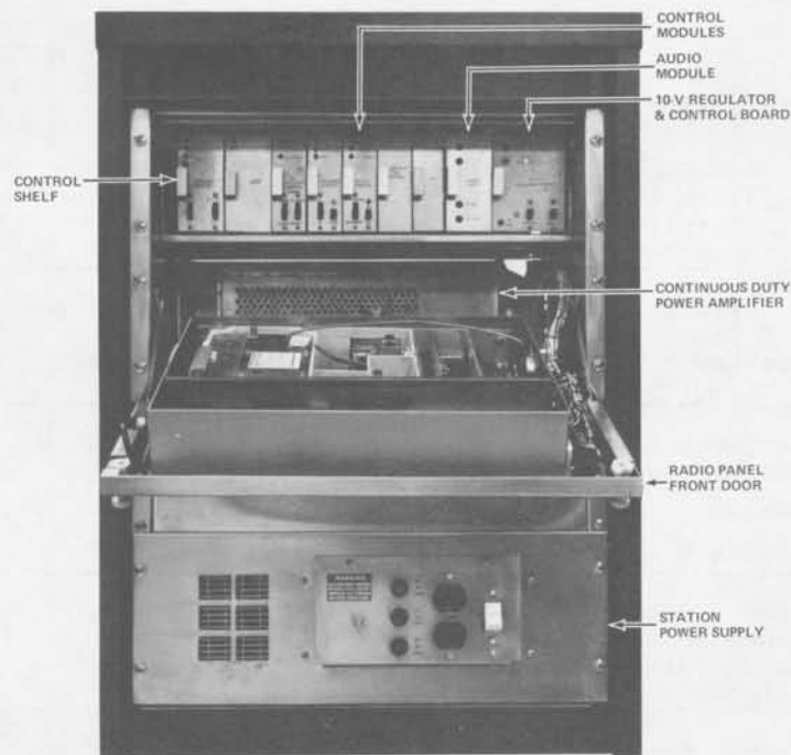
Figure 2 - Station Assemblies
