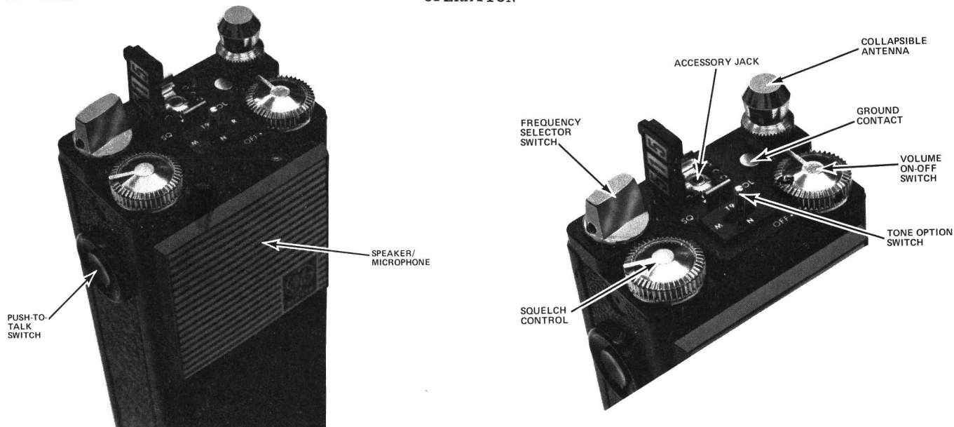
Figure 3 - Operating Controls
