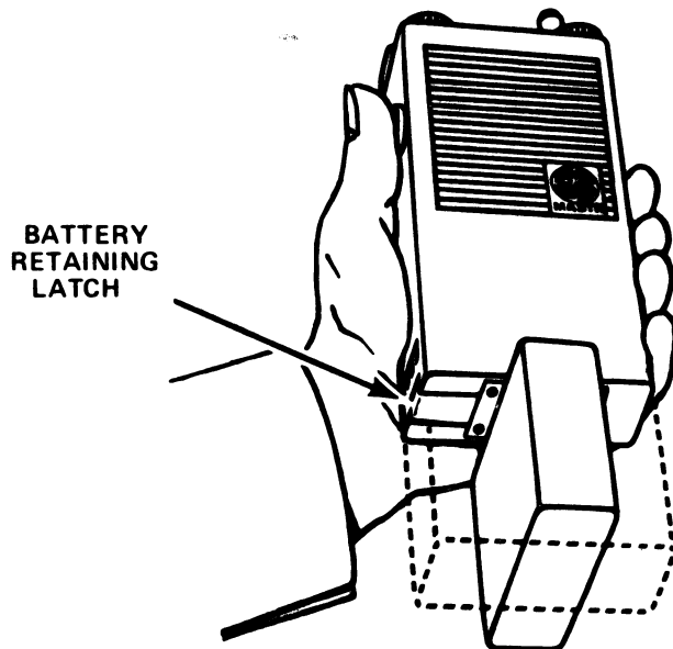
Figure 4 - Battery Pack Replacement
