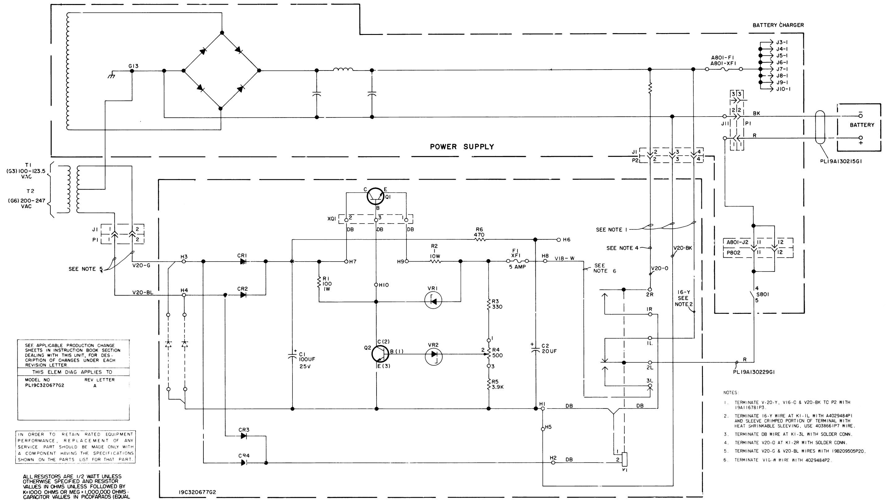
SCHEMATIC DIAGRAM BATTERY STANDBY/CHARGER KITS 19C320677G3 & G6
