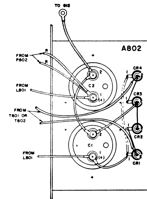
VIEW "B" OUTLINE DIAGRAM
