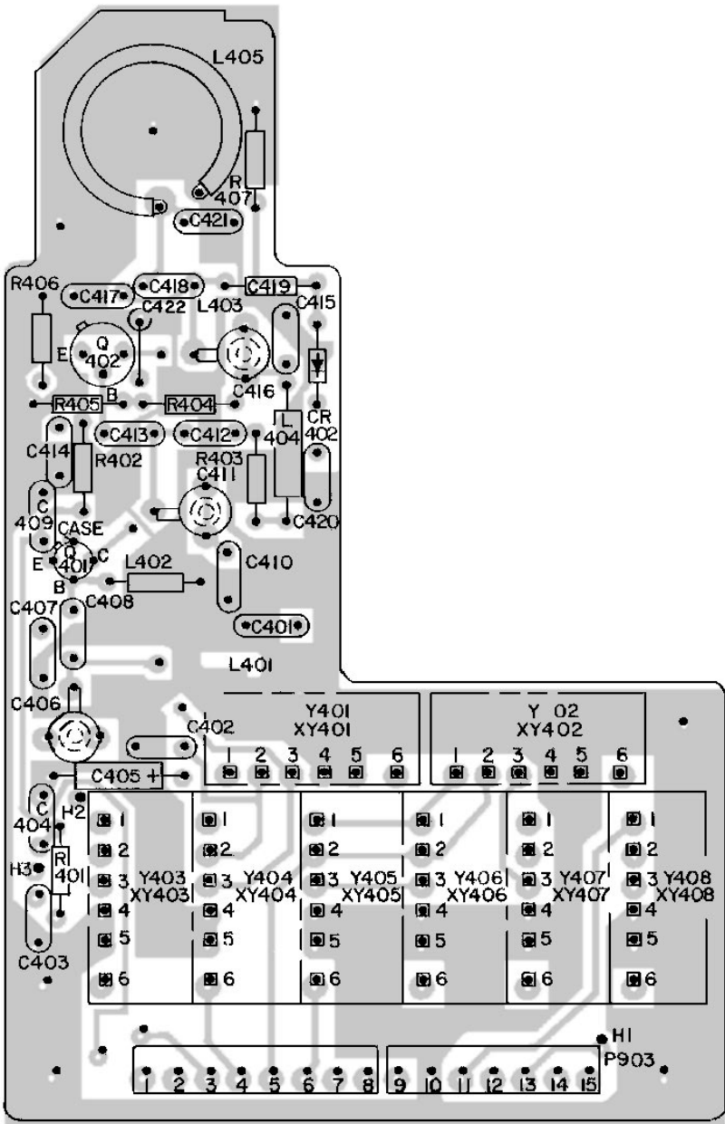
COMPONENT SIDE
