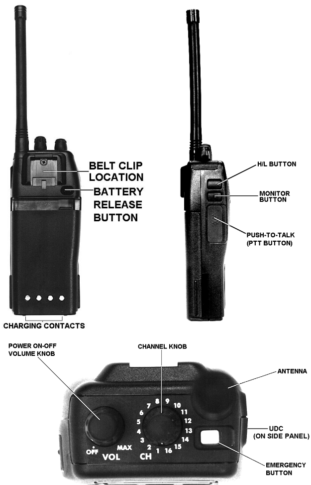
Figure 3 - Top, Back And Left Panel Views
