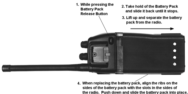
Figure 5 - Installing And Removing The Battery Pack
