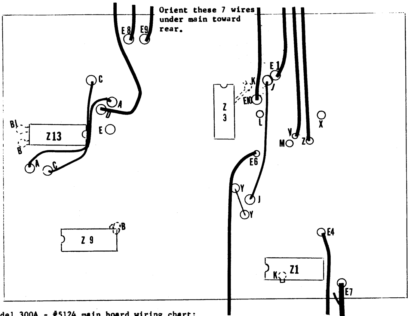
Model 300A - #5124 main board wiring chart: Connect "from" end only at this time.
