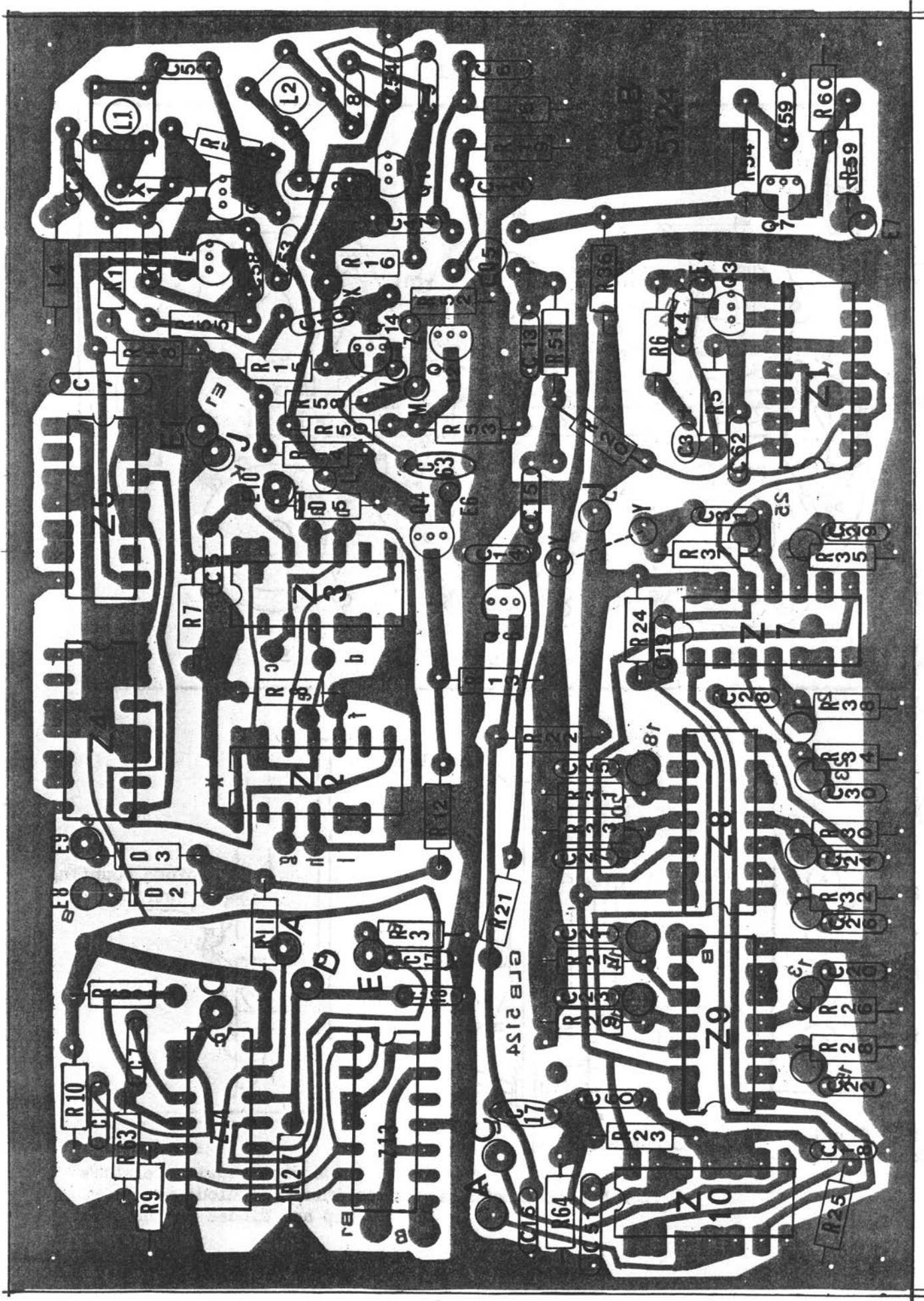
GLB ELECTRONICS #5124 Main Board Layout
