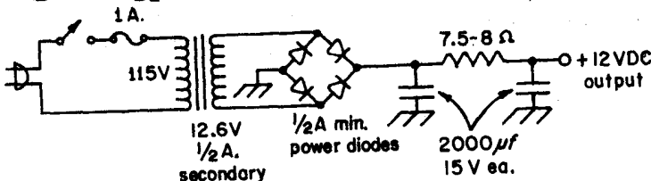
Fig. 6 Suggested circuit for a base-station power supply for the Channelizer.
