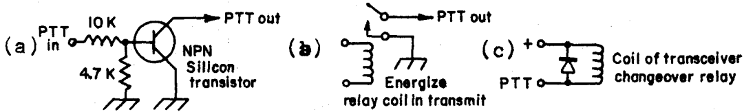
Fig. 1 (a) Circuit for converting positive-going push-to-talk circuits to Channelizer PTT. (b) Use of a relay permits any circuit to be used, as long as the relay can be operated. (c) Showing a "de-spiking" diode across the normal changeover relay in transceiver, when Channelizer PTT line is directly connected.
