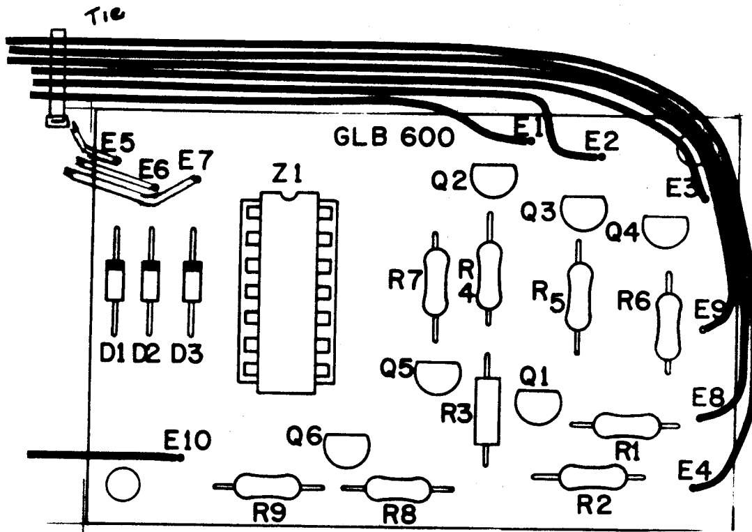
Wiring chart - 600 KHz board
