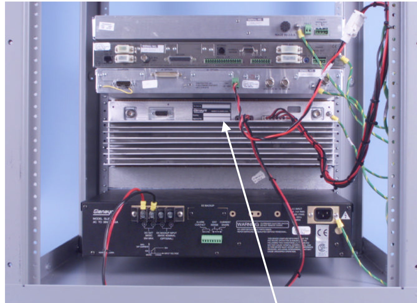
GL-T8200 REAR VIEW WITH FCC LABEL LOCATION
