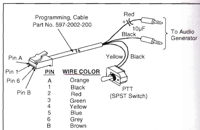
Figure 7-2 Microphone Substitution Fixture
