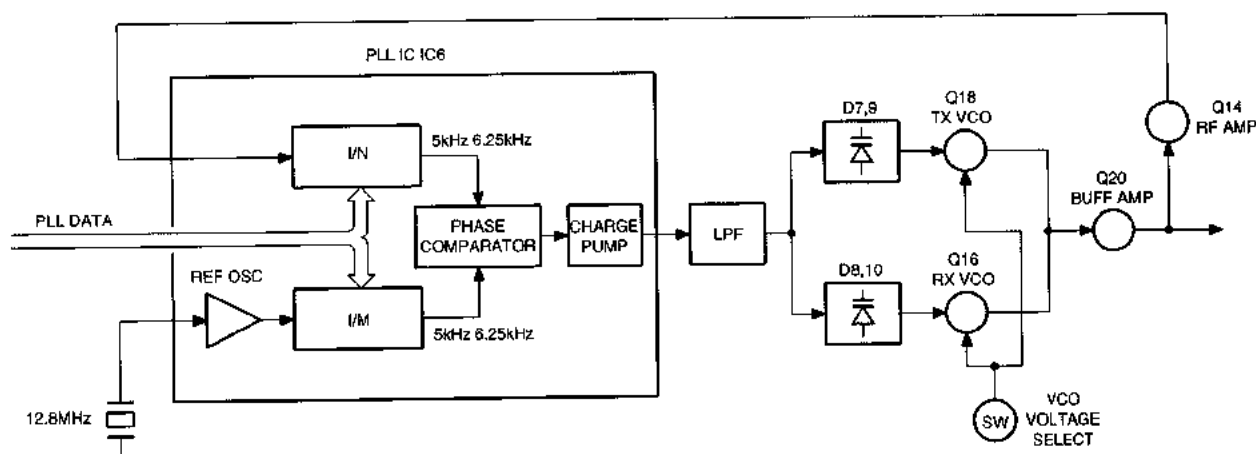
Fig.4 PLL circuit
