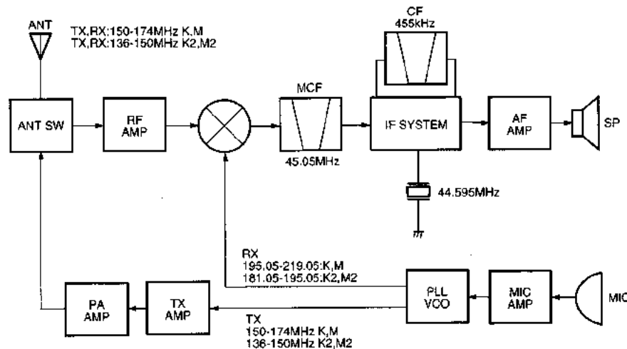
Fig. 1 Frequency configuration
