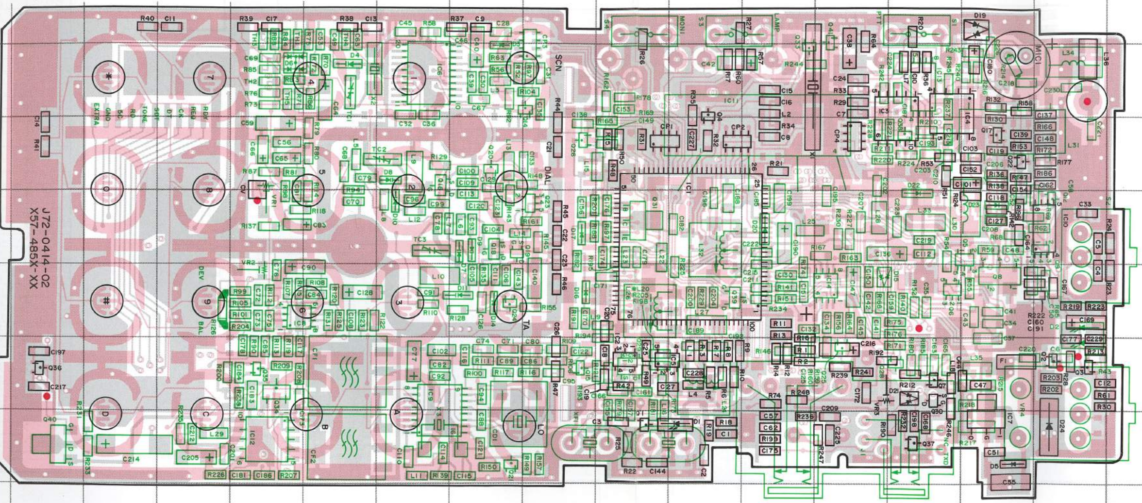
TX-RX UNIT (X57-4850-XX) Component side view + Foil side view -13:K, -14:K2, -20:M, -21:M2
