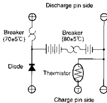
CIRCUIT DIAGRAM
