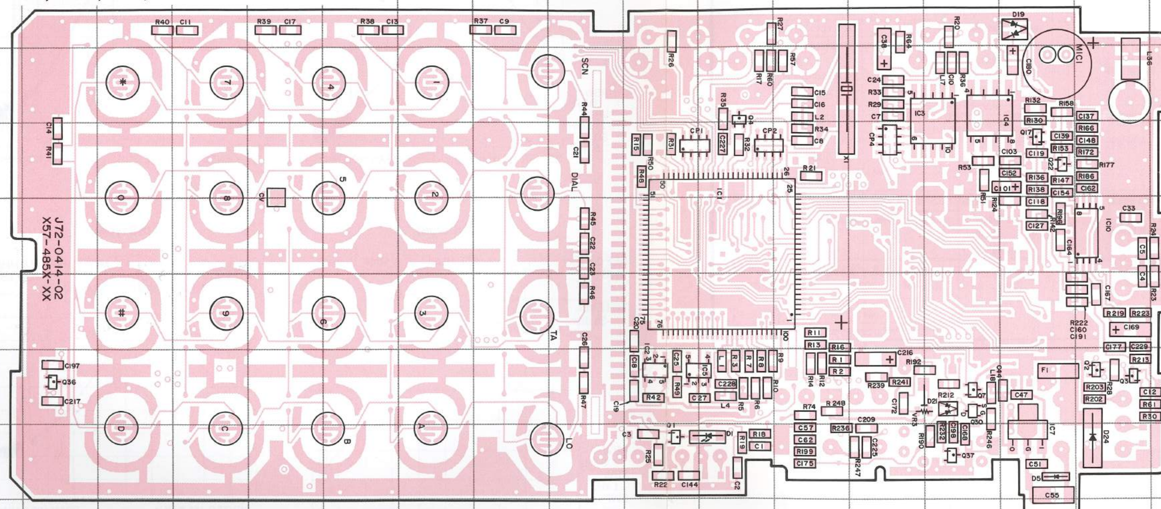
TX-RX UNIT (X57-4850-XX) Component side view -13:K, -14:K2, -20:M, -21:M2
