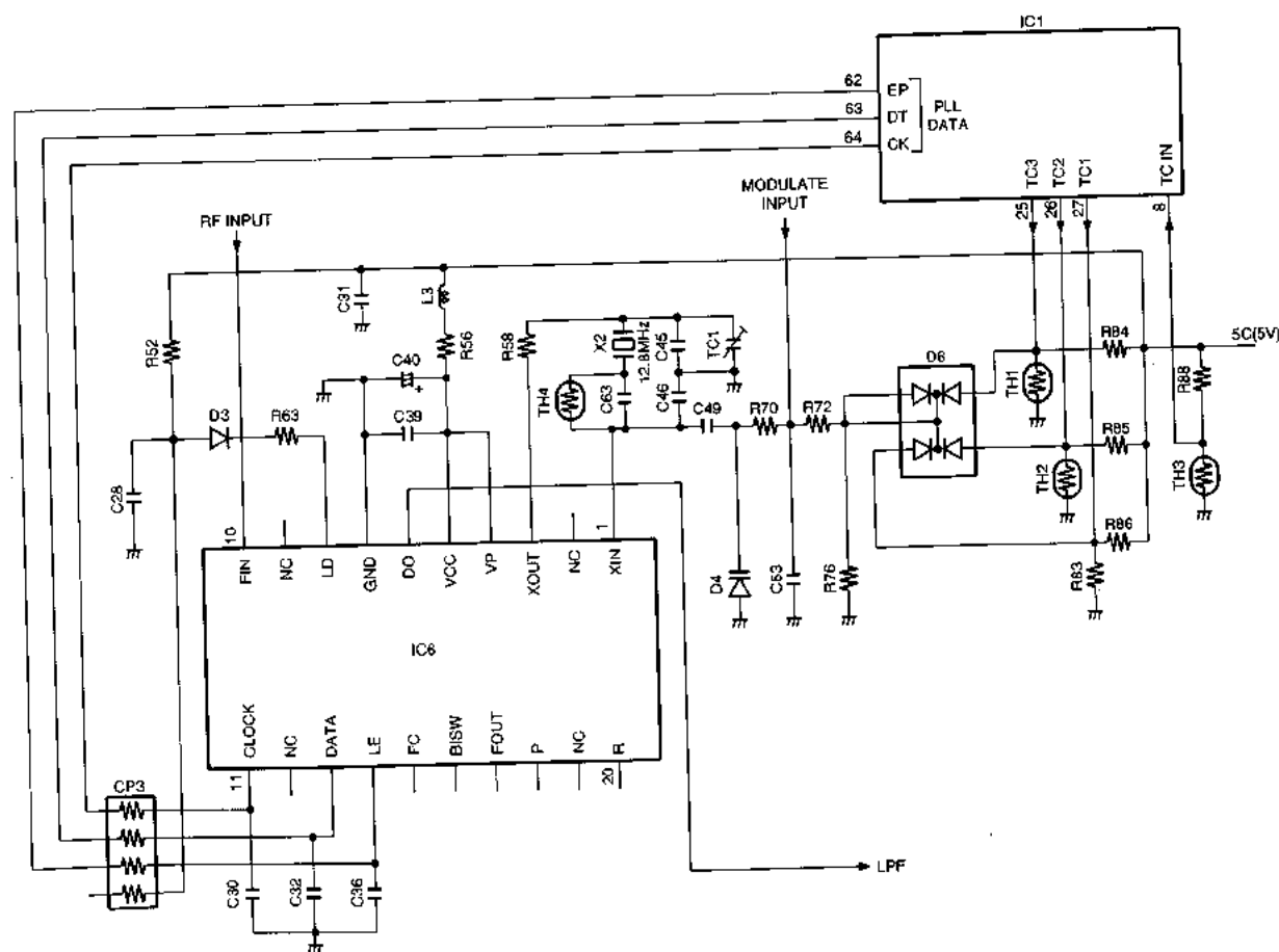
Fig.5 Referend Oscillator circuit
