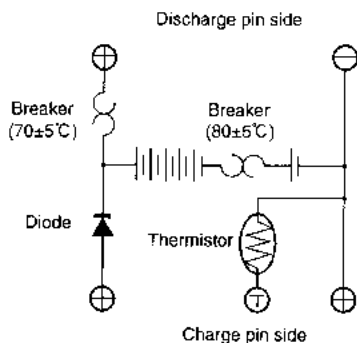
CIRCUIT DIAGRAM
