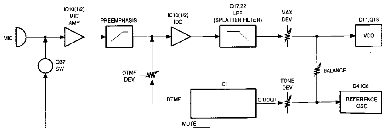
Fig.6 Transmit audio and QT/DQT
