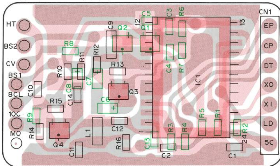
PLL (X58-371X-XX) (A/2) Foil side view
