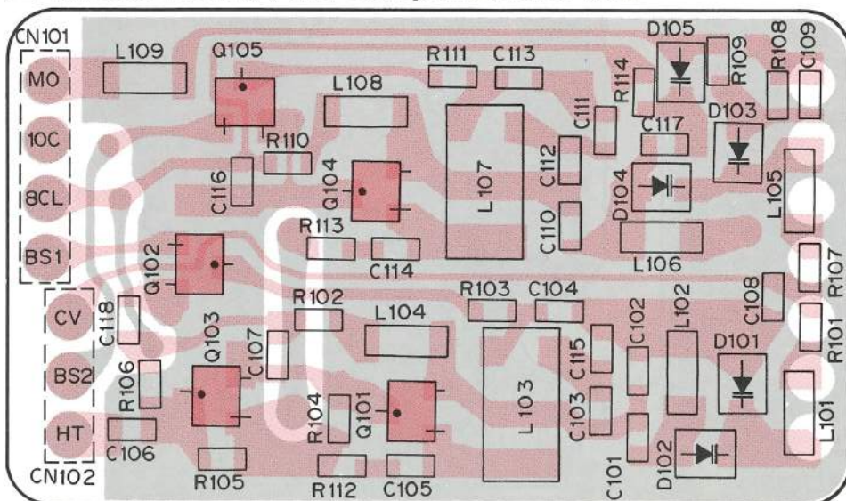
PLL (X58-371X-XX) (B/2) Component side view
