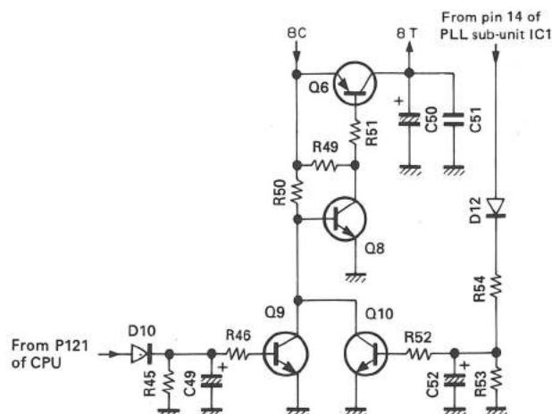
Fig. 5 8T and unlock circuits
