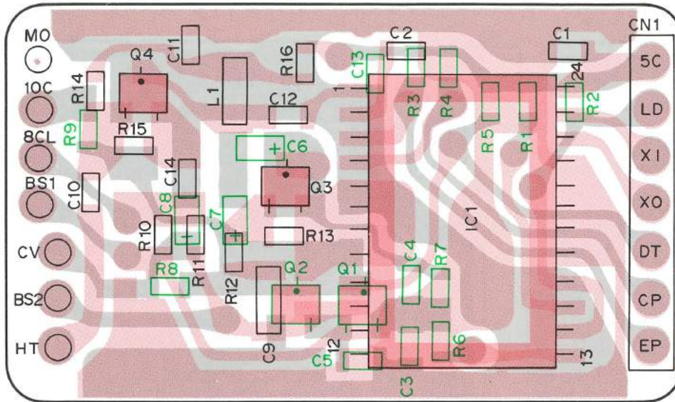
PLL (X58-371X-XX) (A/2) Component side view
