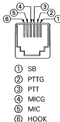
MIC connector front view
