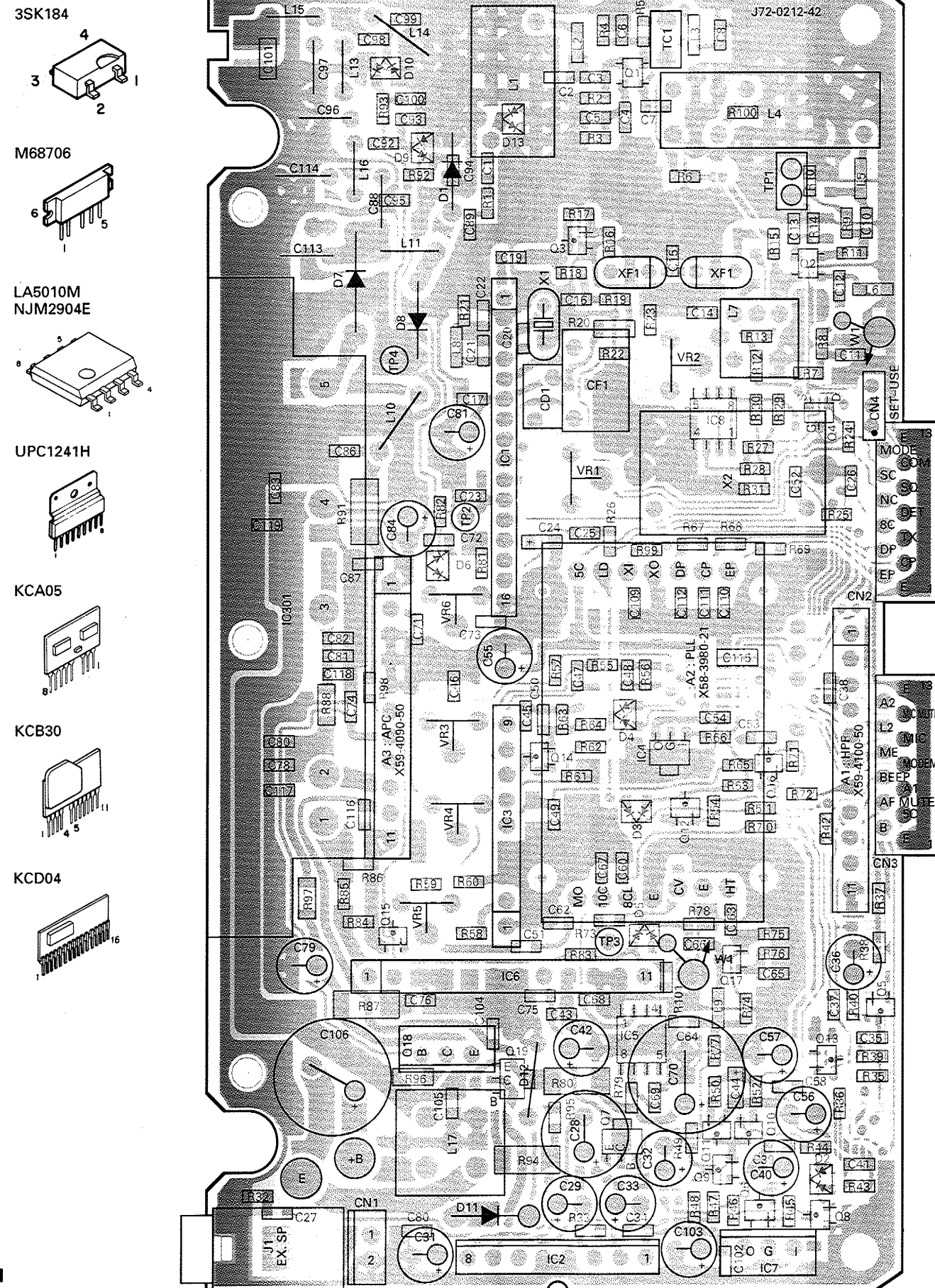
TX-RX UNIT (X57-4250-21) : TK-715(N) (M) Component side view
