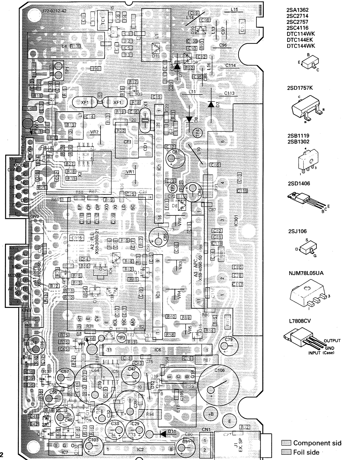
TX-RX UNIT (X57-4250-21) : TK-715(N) (M) Foil side view
