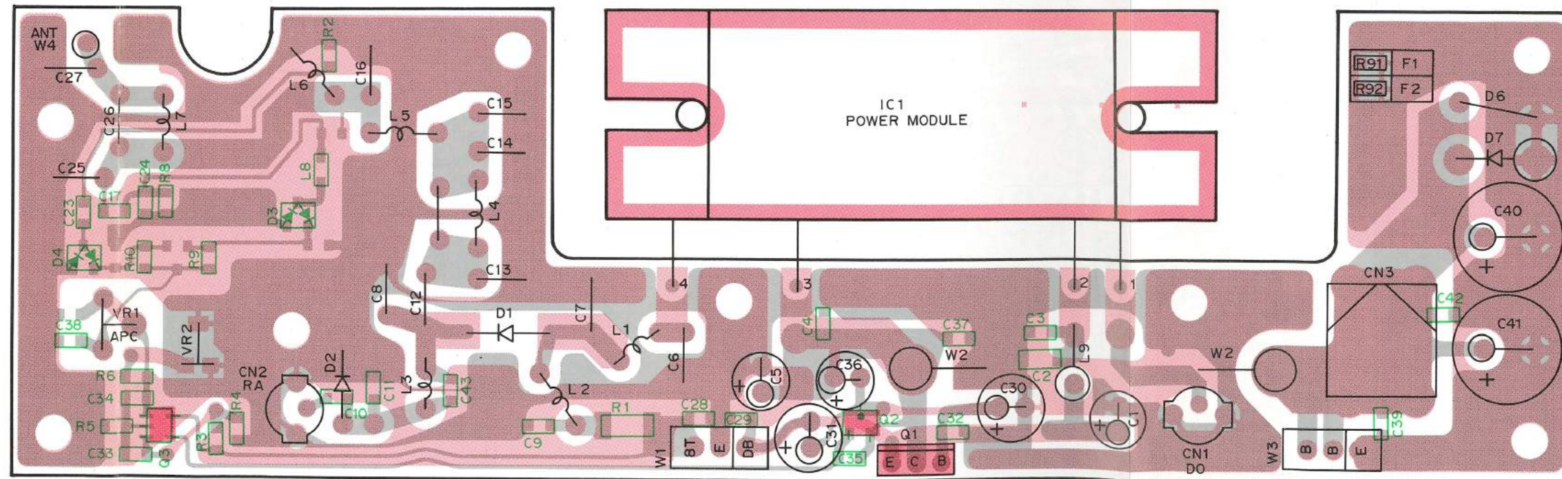
FINAL UNIT (X57-3750-XX) (D/4) -11 : K,M -12 : K2,M2 Foil side view
