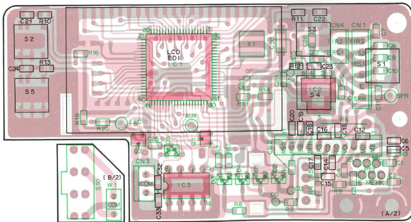
DISPLAY UNIT (X54-3100-20) : KCH-3 Foil side view
