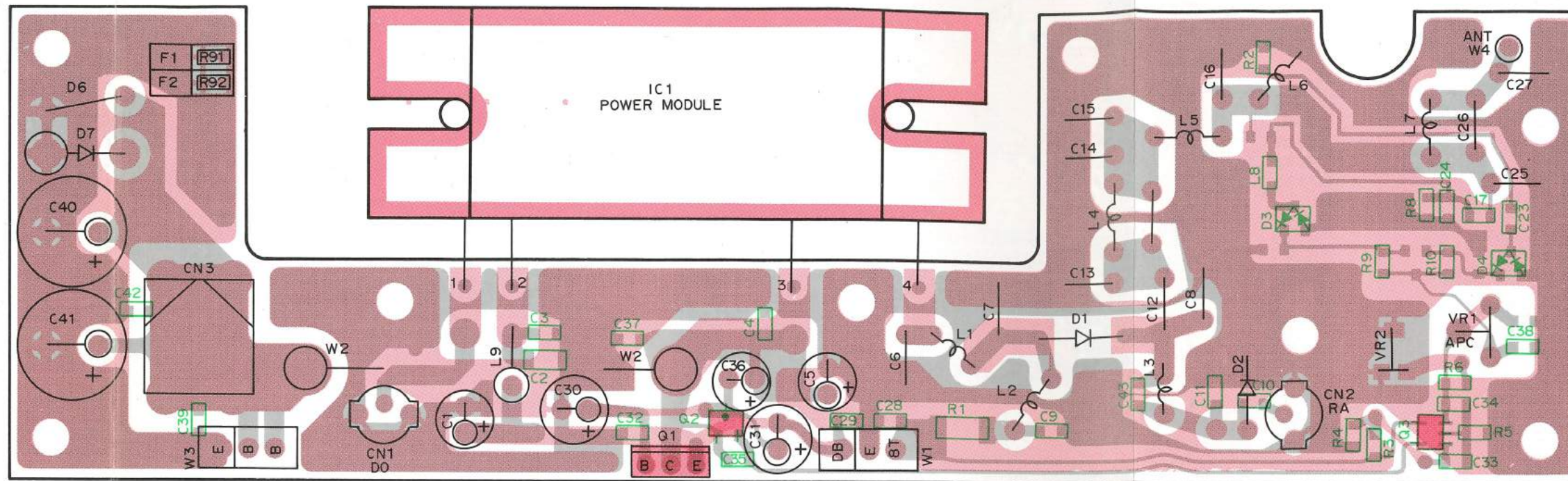
FINAL UNIT (X57-3750-XX) (D/4) -11 : K,M -12 : K2,M2 Component side view
