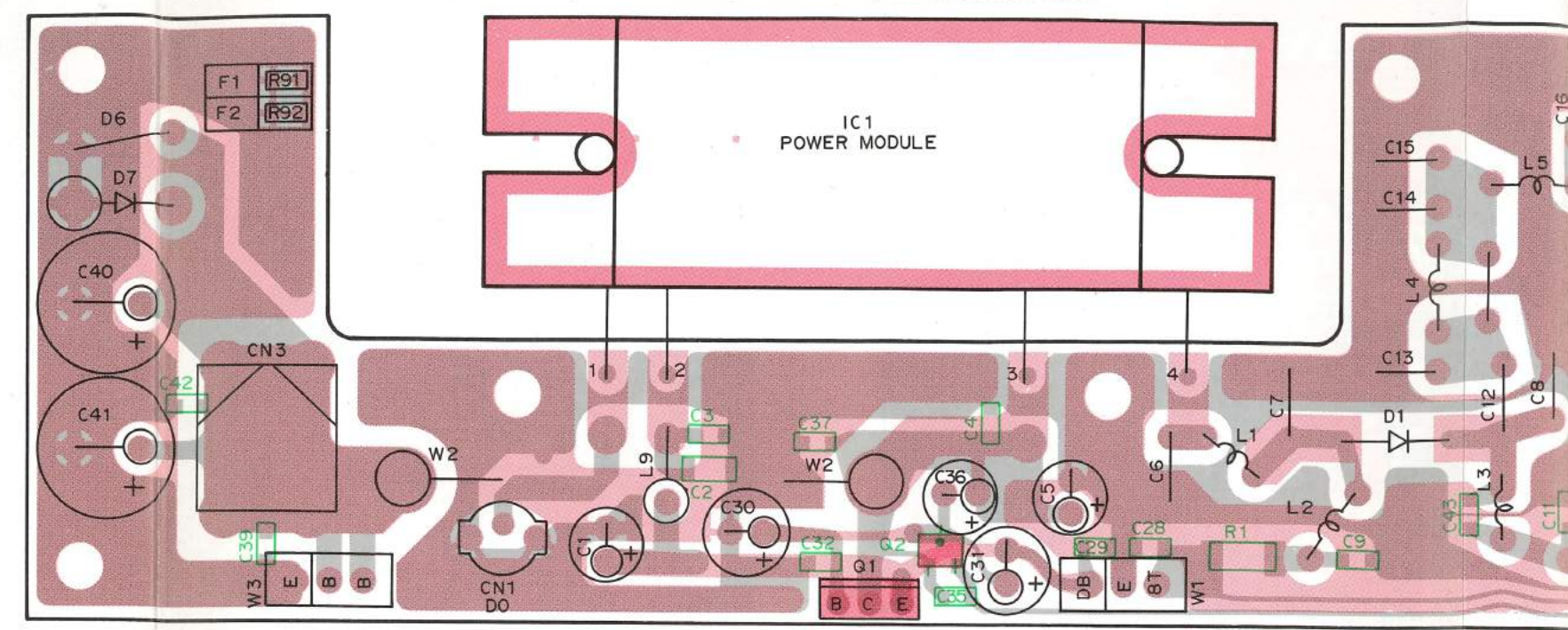
FINAL UNIT (X57-3750-XX) (D/4) -11 : K,M -12 : K2,M2 Component side view
