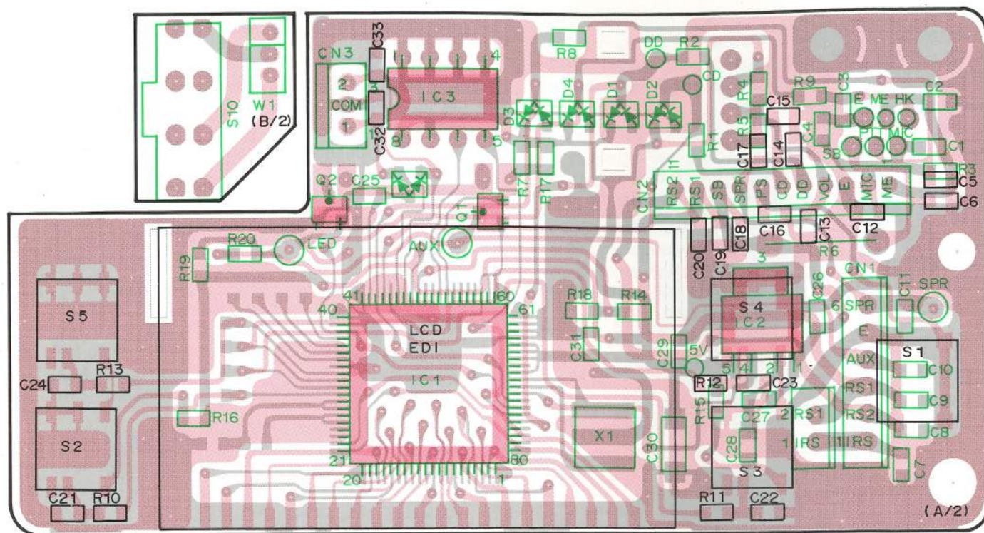
DISPLAY UNIT (X54-3100-20) : KCH-3 Component side view
