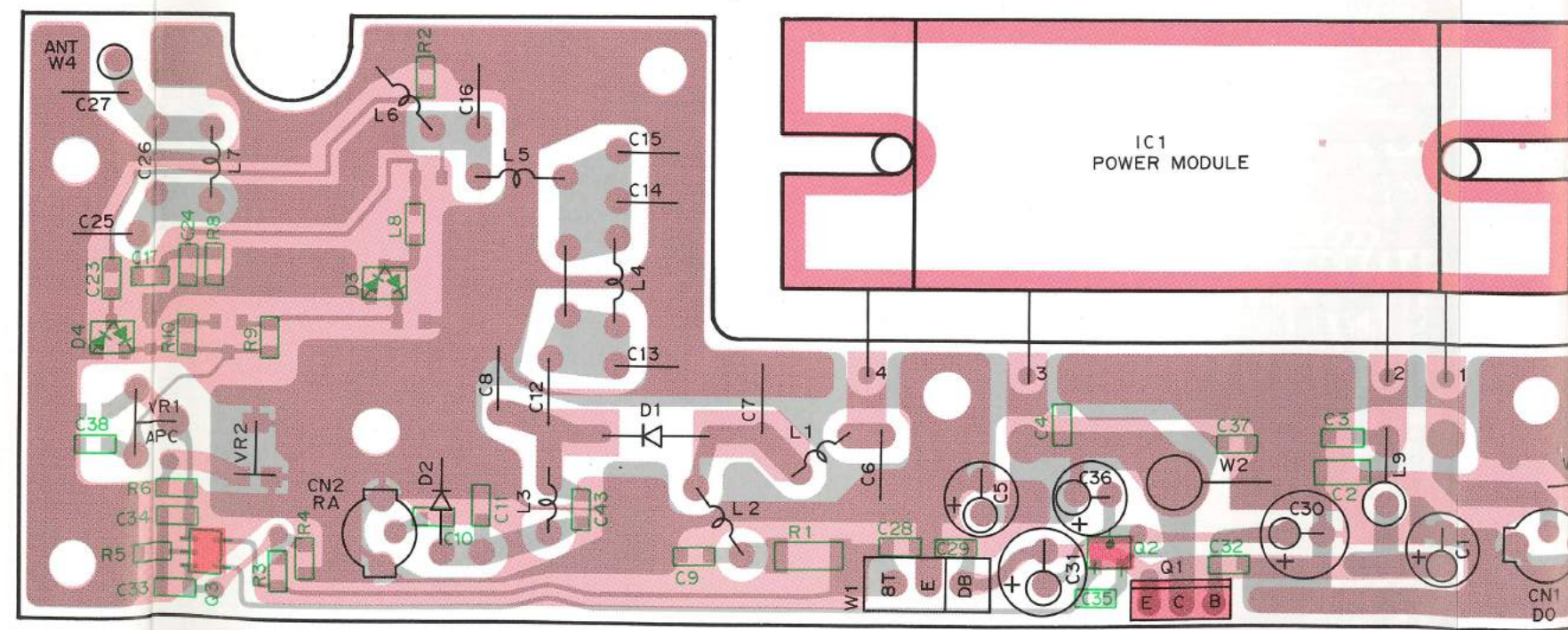
FINAL UNIT (X57-3750-XX) (D/4) -11 : K,M -12 : K2,M2 Foil side view
