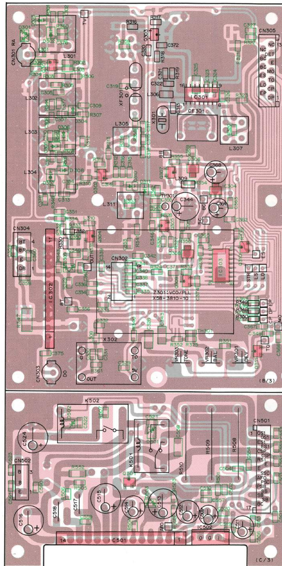
TX-RX UNIT (X57-3750-10) Component side view
