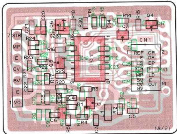
VCO/PLL UNIT (X58-3810-10) Foil side view
