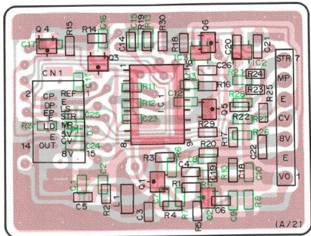
VCO/PLL UNIT (X58-3810-10) Component side view
