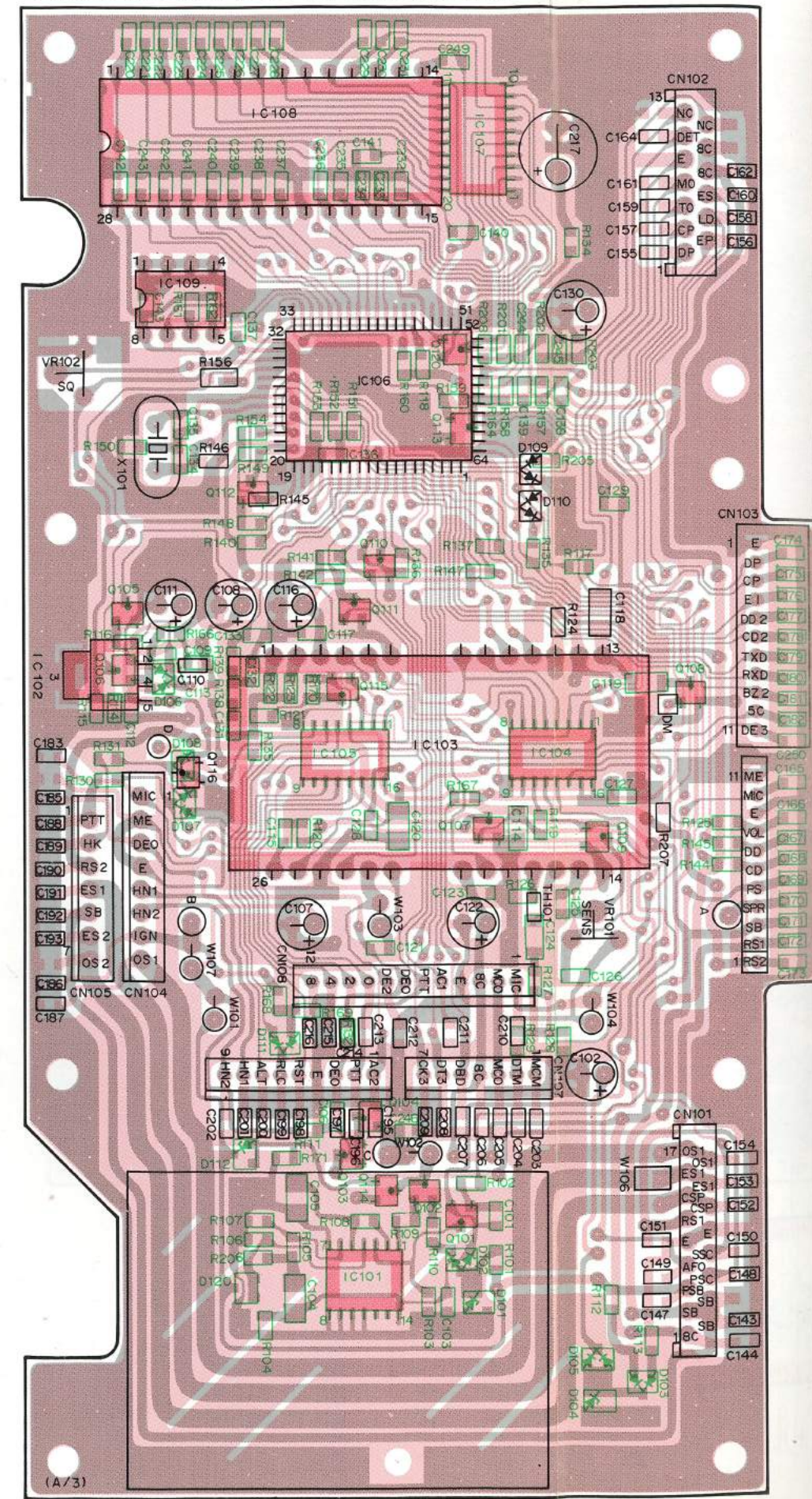
TX-RX UNIT (X57-3750-10) Foil side view
