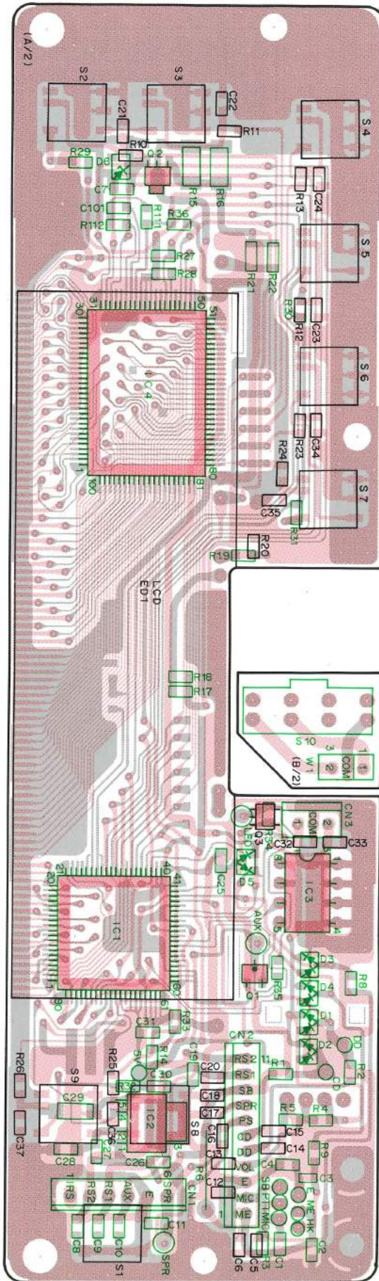
DISPLAY UNIT (X54-3110-20) : KCH-4 Component side view
