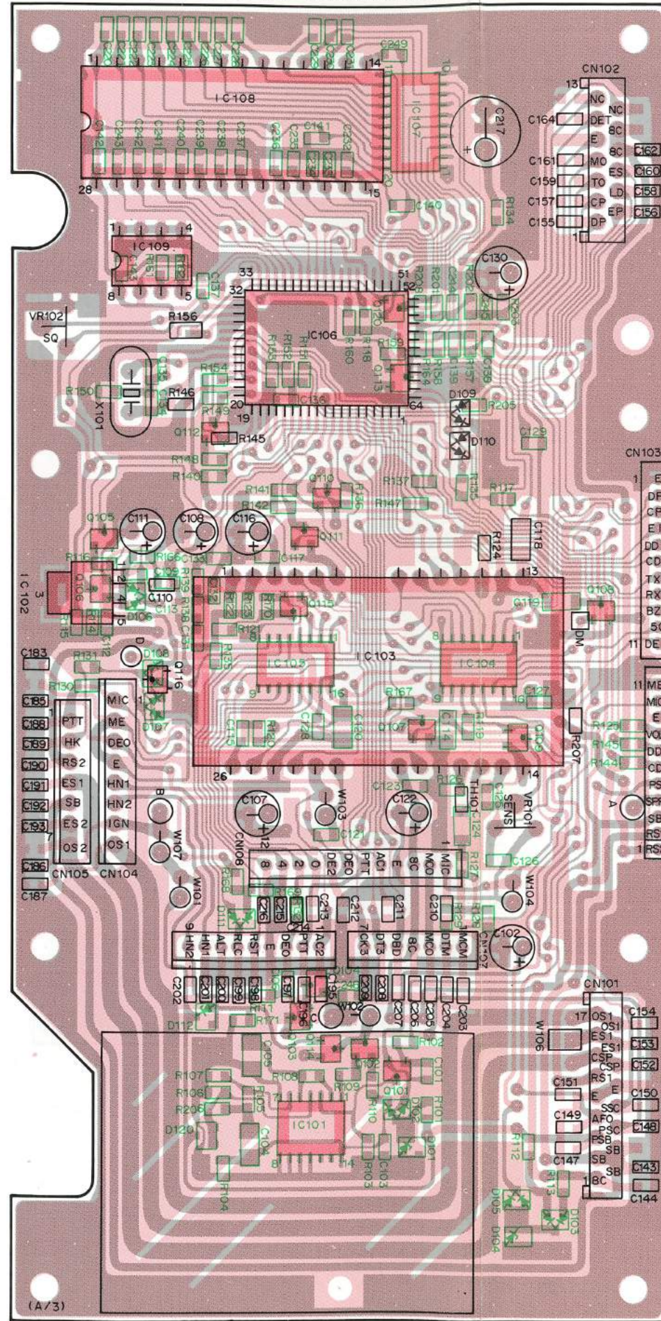
TX-RX UNIT (X57-3750-10) Foil side view
