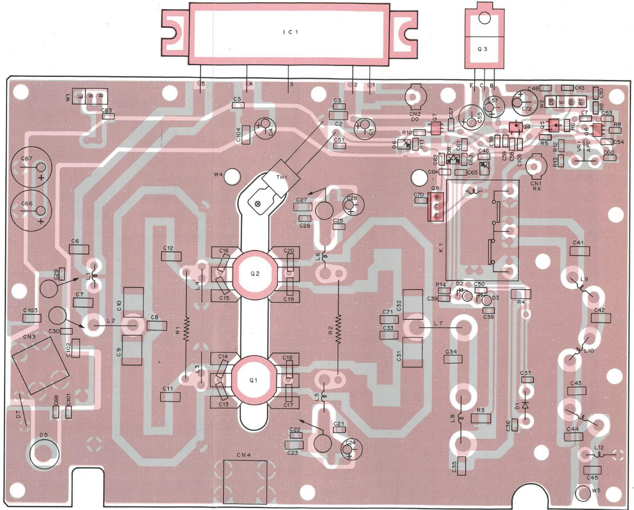
FINAL UNIT (X45-3390-10) Foil side view
