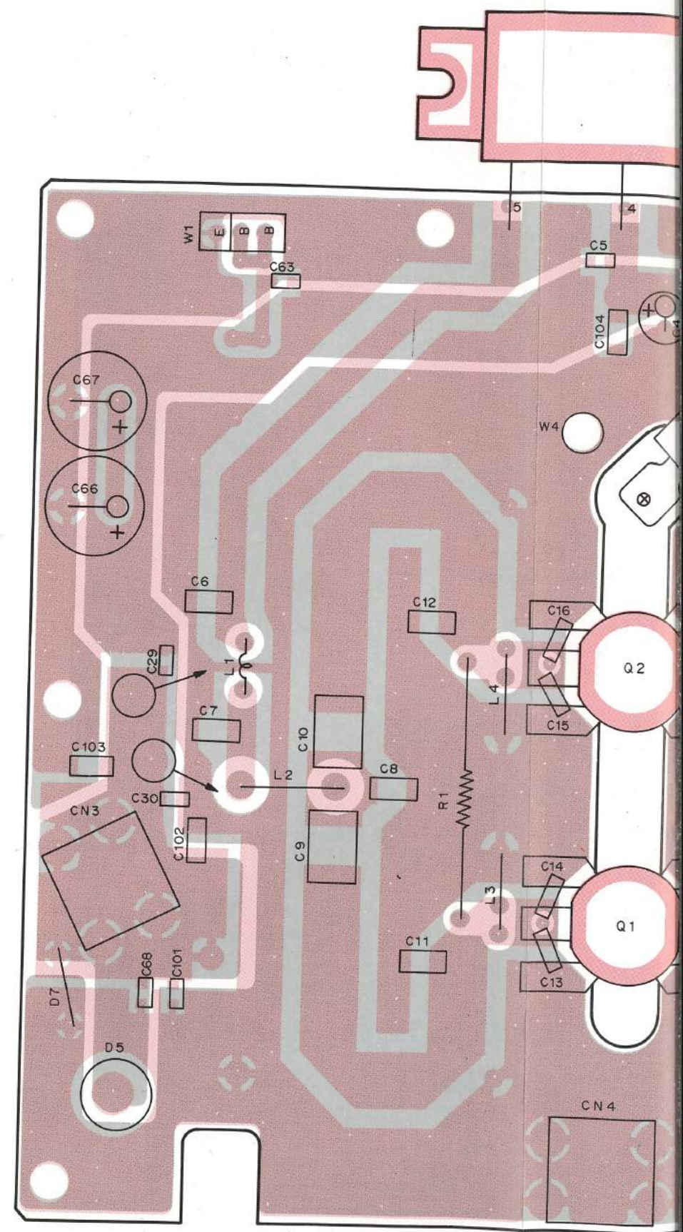
FINAL UNIT (X45-3390-10) Foil side view
