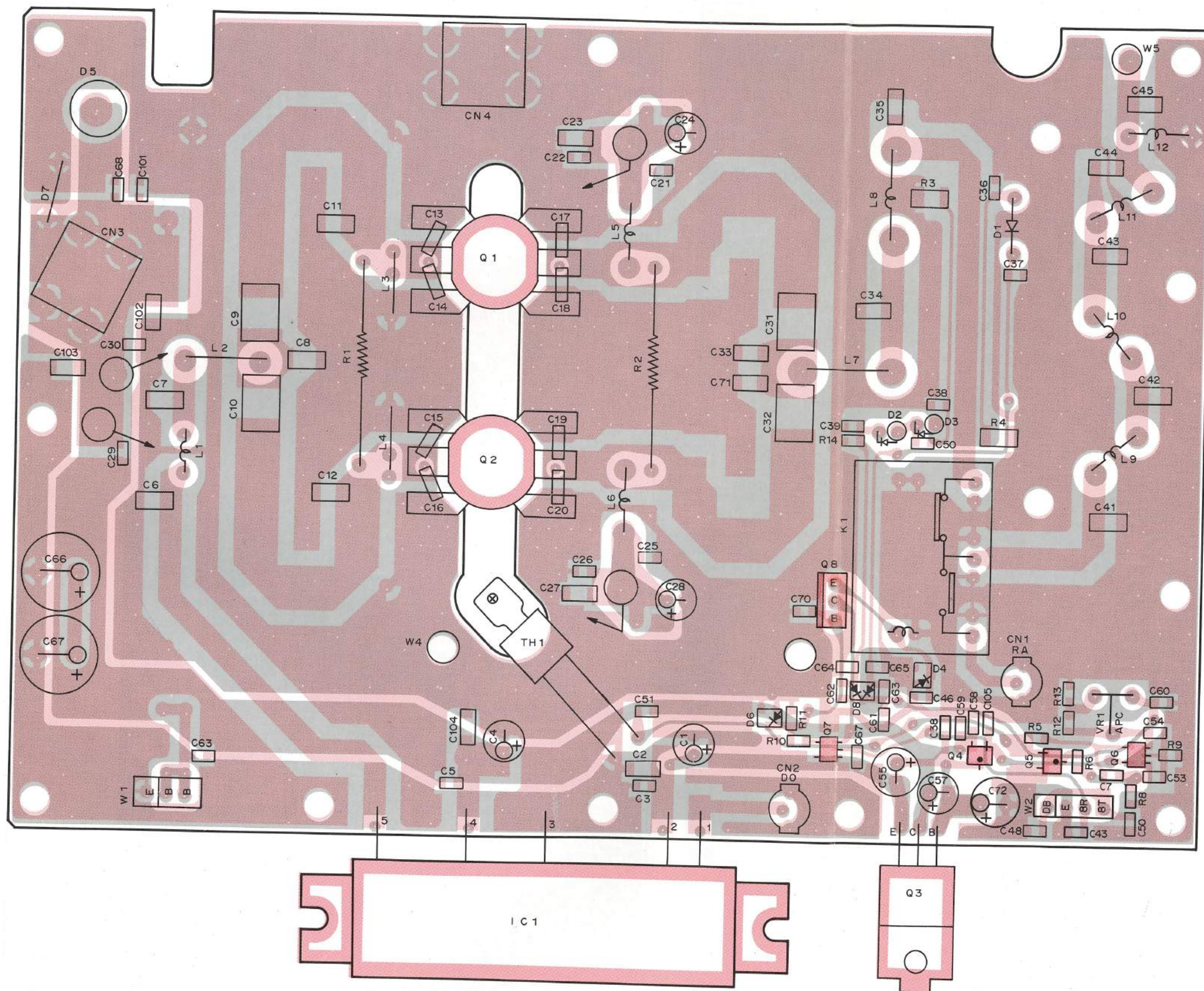
FINAL UNIT (X45-3390-10) Component side view
