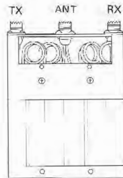
CELWAVE'S Duplexer
