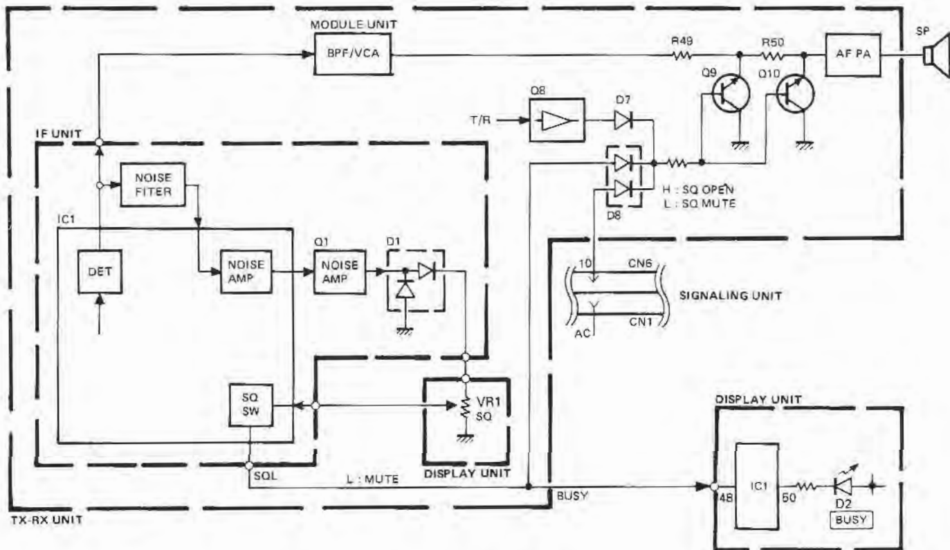
Fig. 3 Squelch circuit
