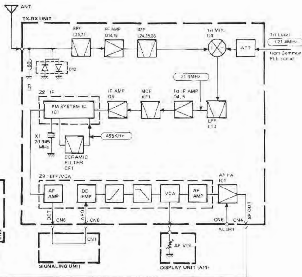
Fig. 2 Receiver block diagram
