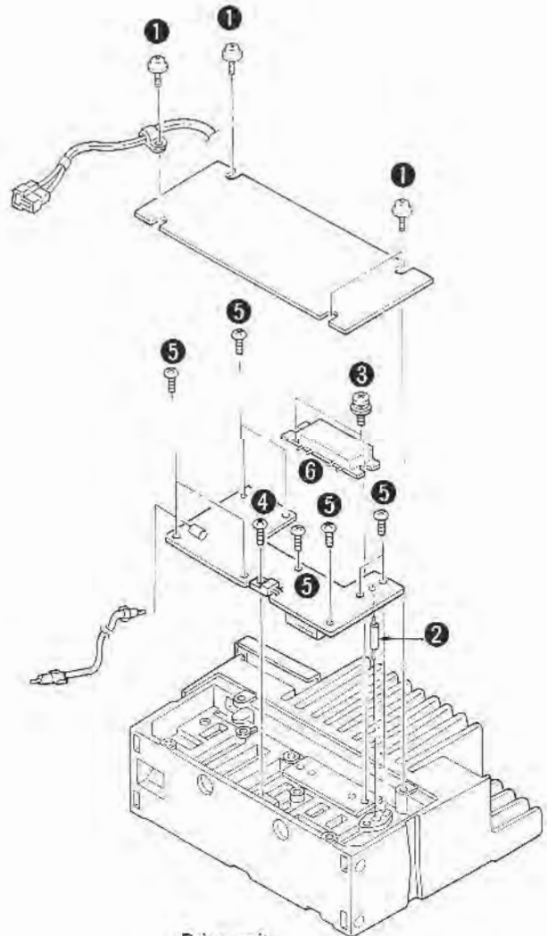
Drive unit
