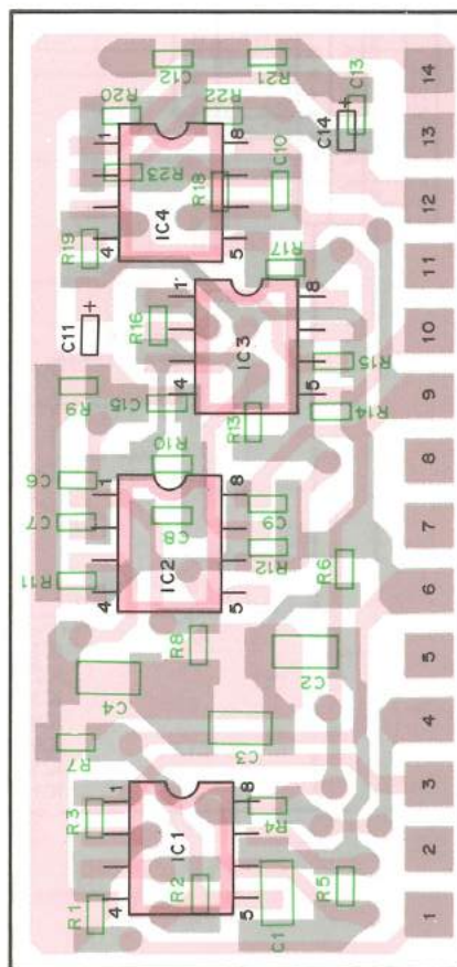
Component side view
