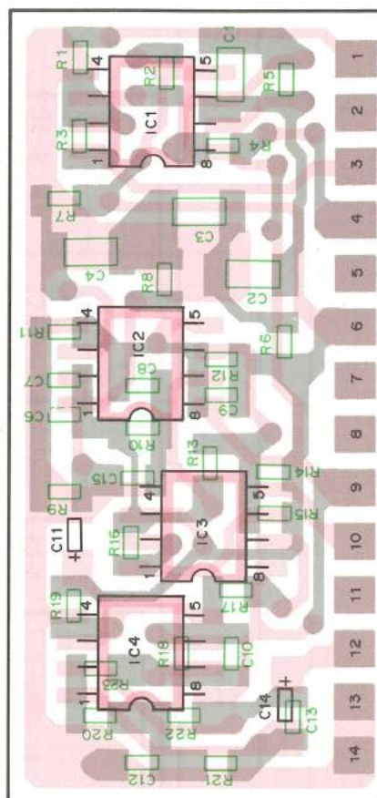
Foil side view
