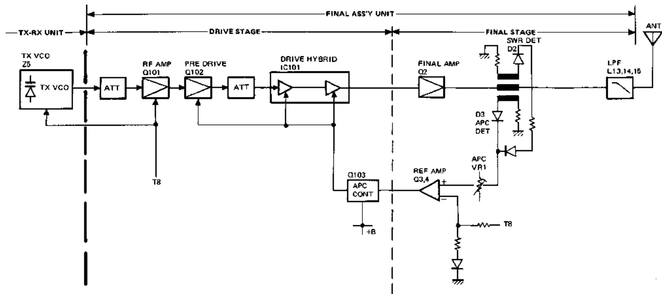
Fig. 1 Transmitter block diagram
