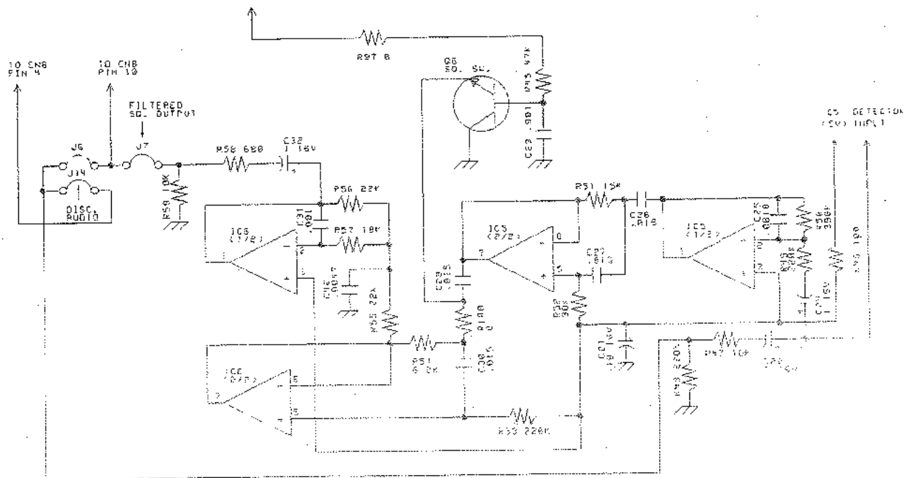
MODIFIED CIRCUIT
