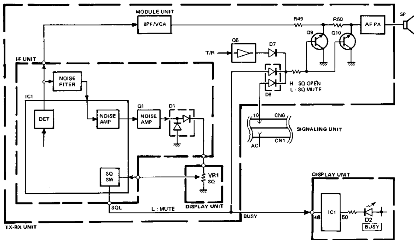
Fig. 3 Squelch circuit
