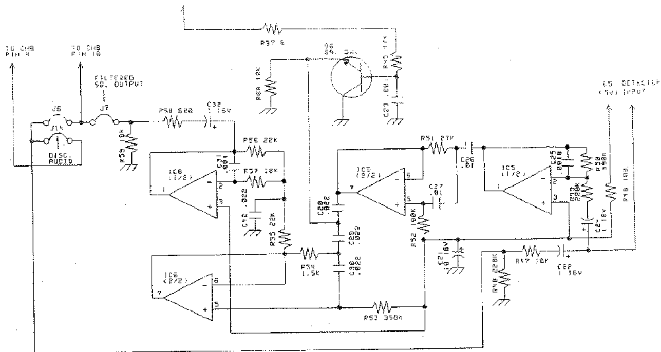
ORIGINAL CIRCUIT
