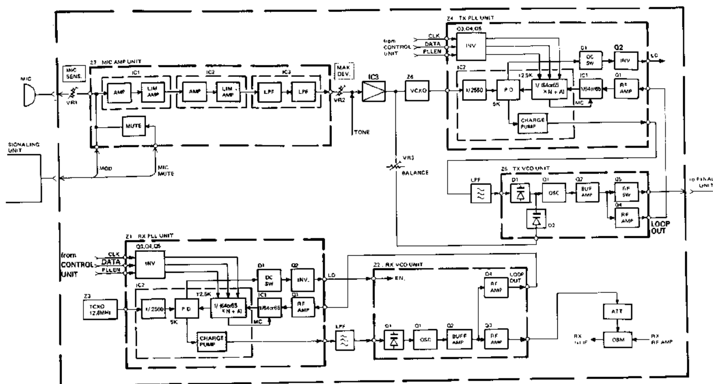
Fig. 4 PLL & Modulation circuit block diagram
