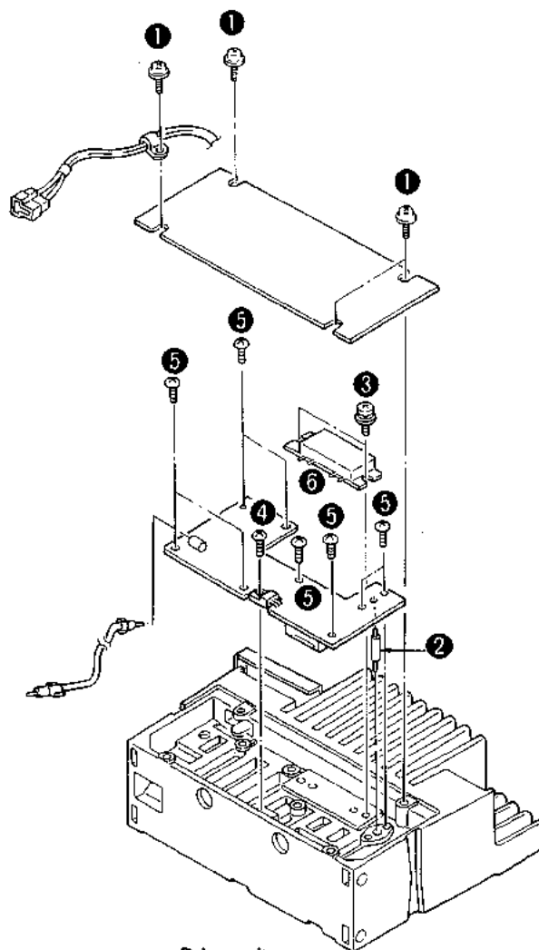
Drive unit
