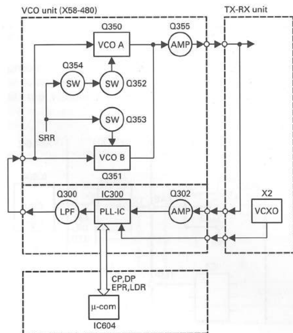
Fig. 5 Receiver PLL
