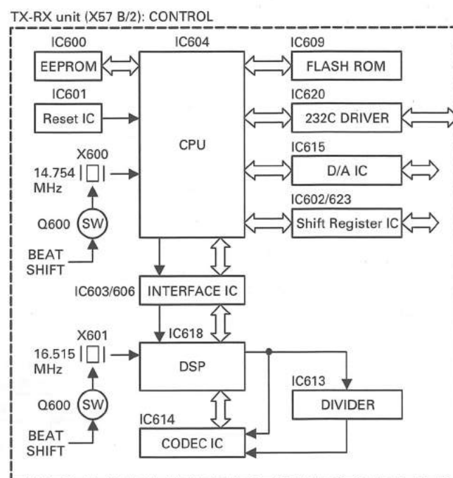
Fig. 8 Control circuit
