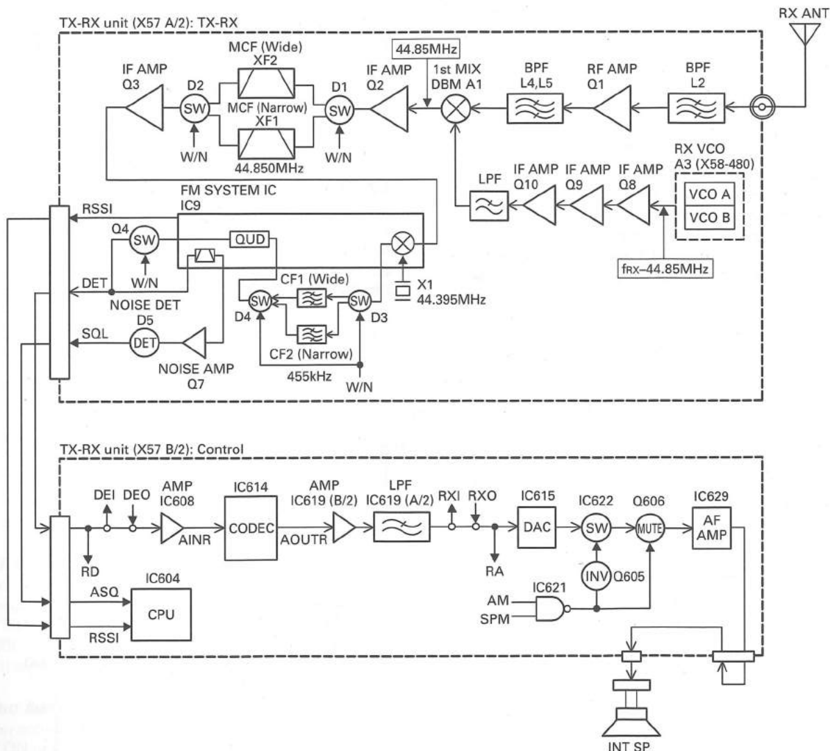
Fig. 1 Receiver circuit
