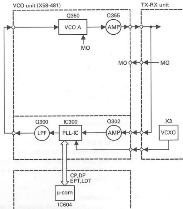
Fig. 6 Transmitter PLL
